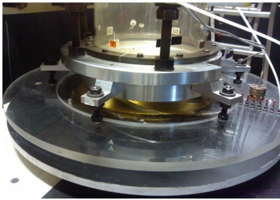
(a) Vaneless diffuser of the centrifugal pump
