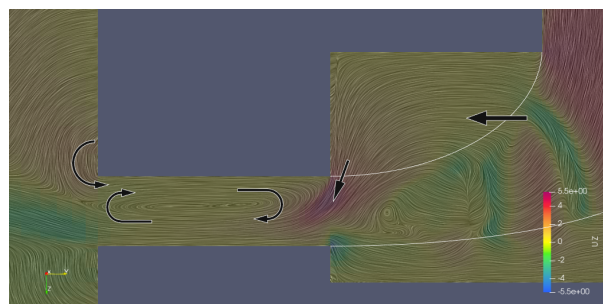
Figure 2.22: Formation of the recirculation bubble in the diffuser
