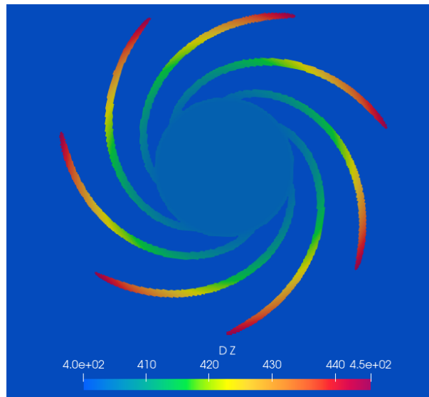
Figure 2.21: Radial expansion of Dz over the impeller radius
