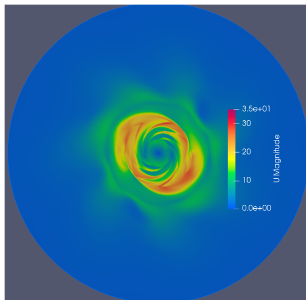
Figure 2.19: Velocity field for Dx = 4e7 and Dy = 2e7
