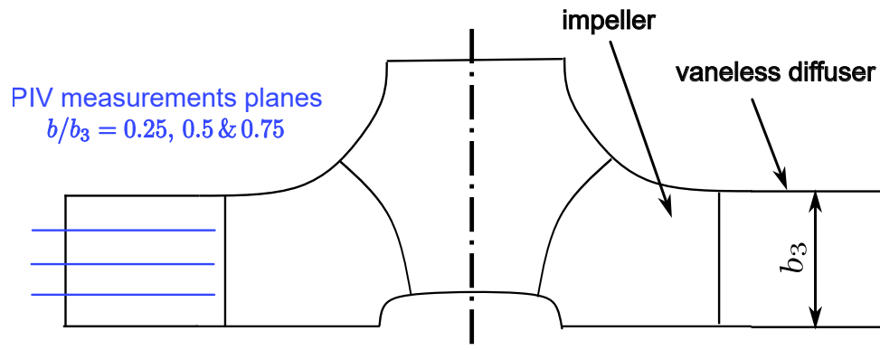
Figure 2.8: Position of the PIV plans
