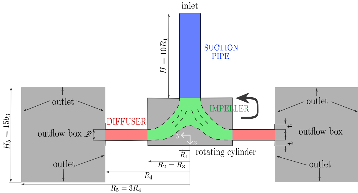
Figure 2.13: Model of the RESDA benchmark
