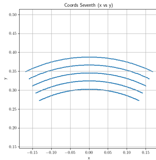
Figure 2.14: Interpolation points over 360/7 degrees
