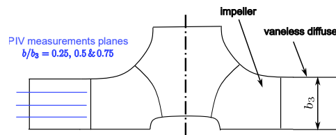
Figure 2.9: Position of the PIV plans
