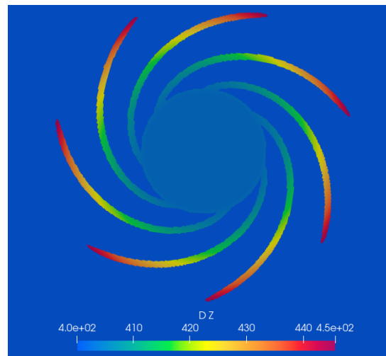
Figure 3.9: Example of a radial expansion of Dz over the impeller radius
