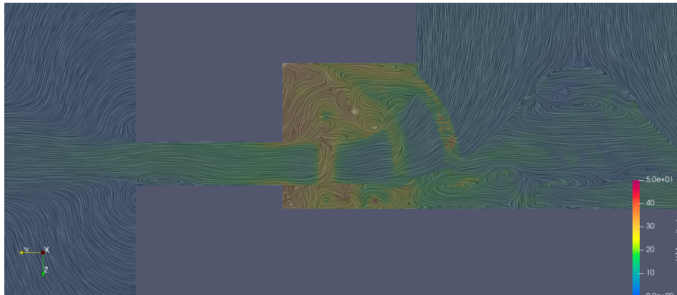
(b) Velocity field obtained a few iterations after releasing the \omega r enforcement
