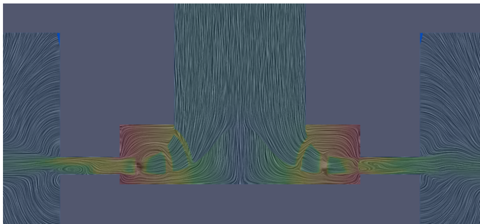
(c) Velocity field obtained long after releasing the \omega r enforcement, confirming the sustained suppression of the recirculation bubble
