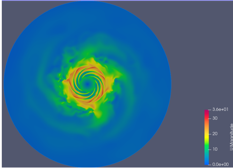
Figure 3.7: Velocity field for Dx = Dy , with high parameters causing the simulation to diverge
