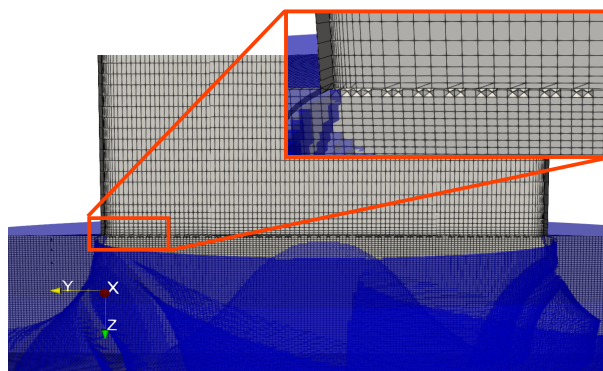
Figure 2.17: Mesh interface between the pipe and the impeller
