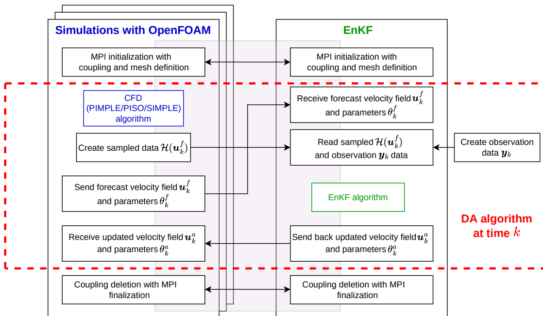
Figure 2.16: CONES structure
