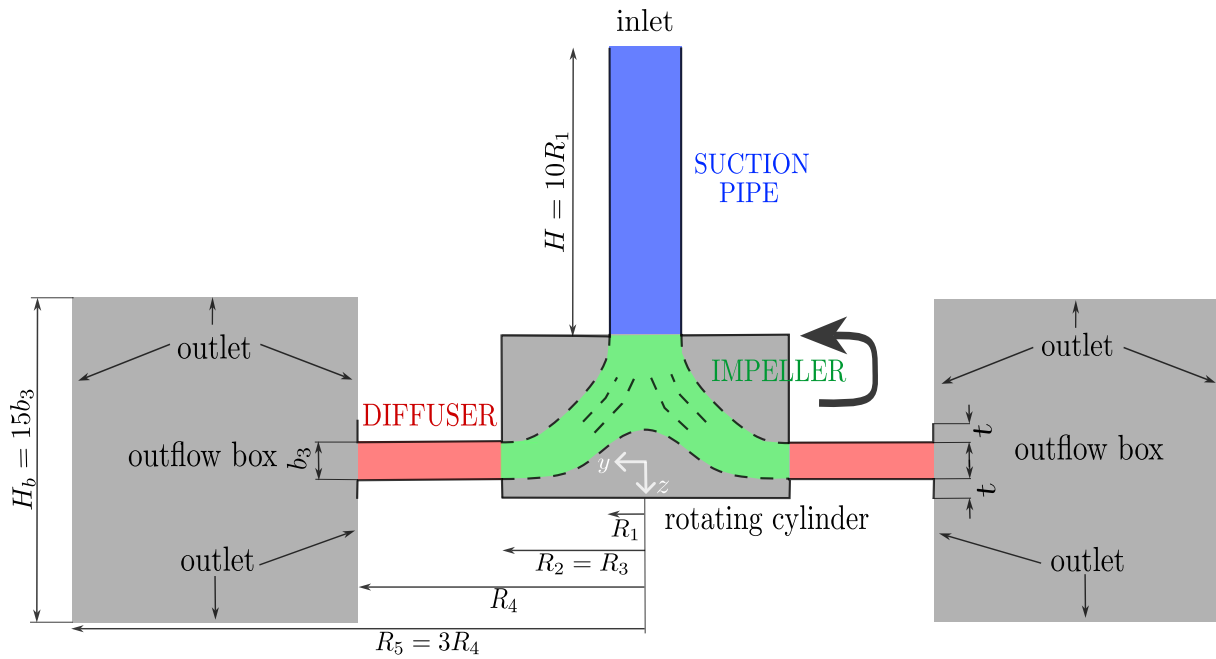
Figure 2.18: Model of the RESDA benchmark
