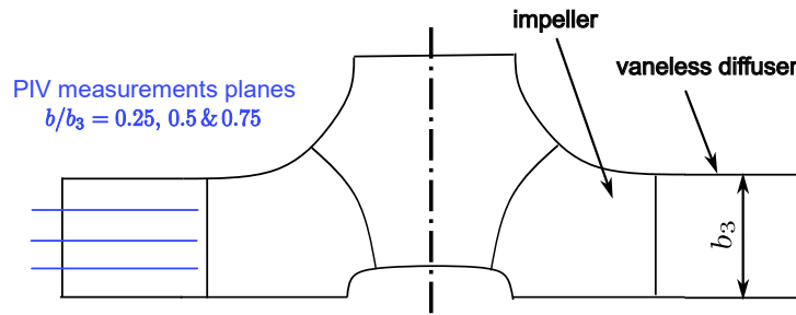
Figure 2.7: Position of the PIV planes on the diffuser
