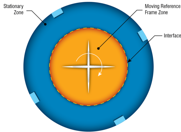
Figure 2.11: MRF Model
