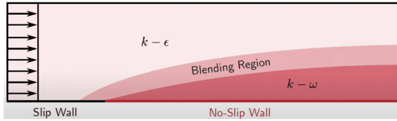
Figure 2.10: k - \omega SST model
