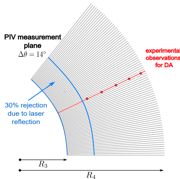
Figure 2.8: Position of the PIV points on a polar slice of the diffuser
