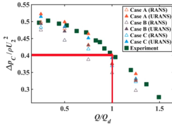
Figure 2.21: Overall pump performance versus reduced pump flow rate Q
