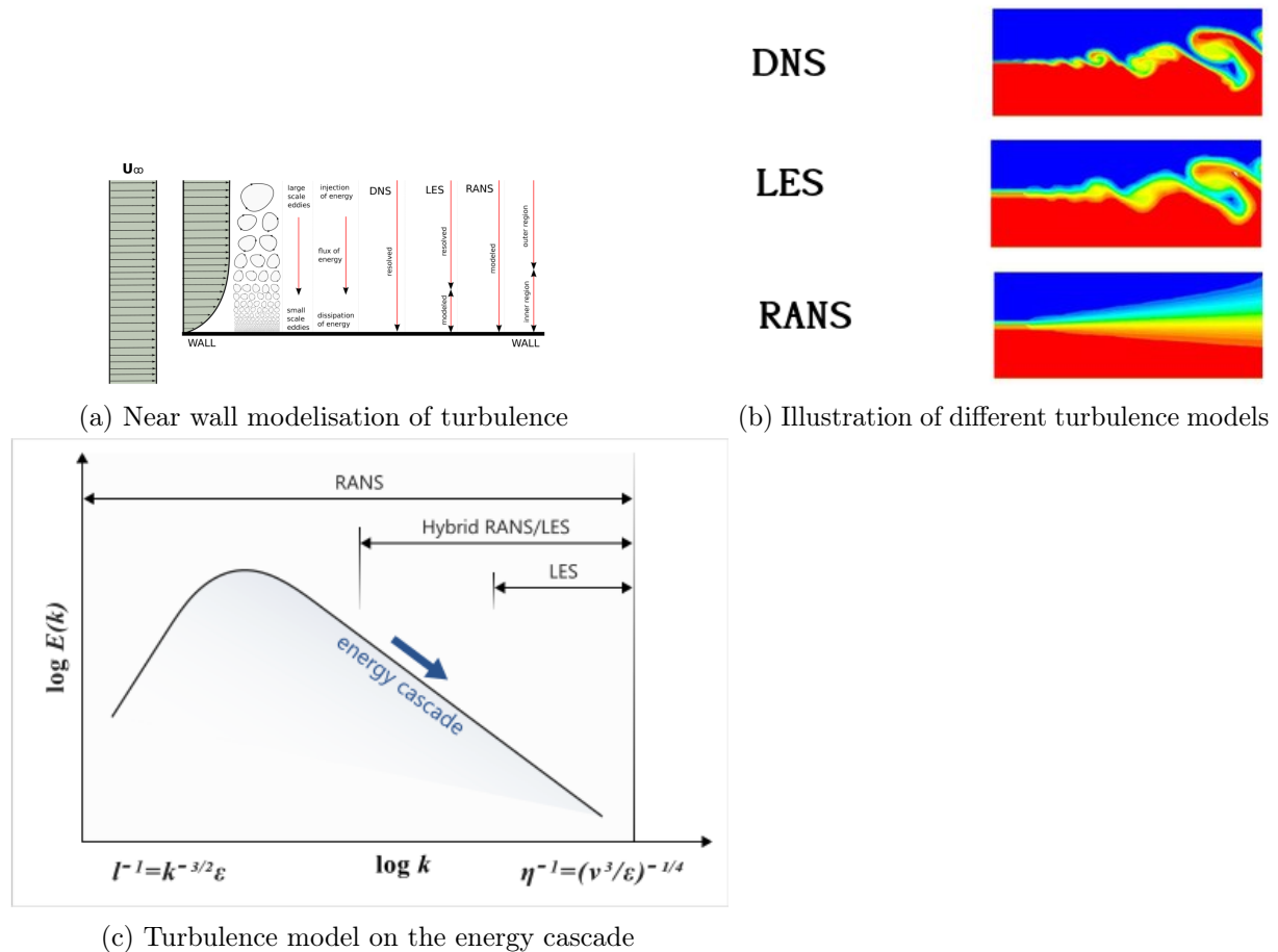
Figure 2.9: Turbulence models
