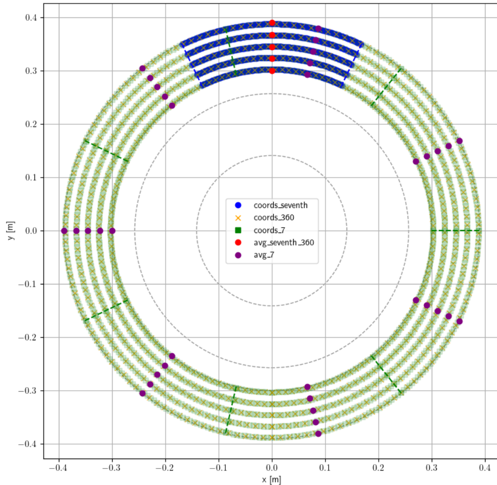
Figure 3.11: Illustration of the augmented coordinates for the interpolation of the field
