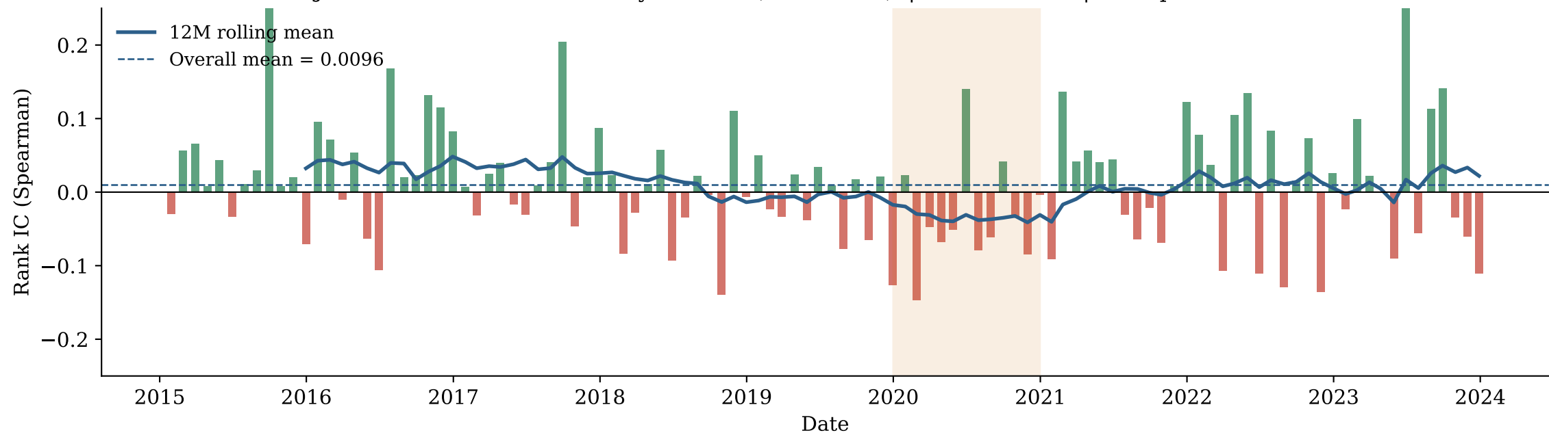
JKP+FinBERT w10×: Monthly Rank IC (2015-2023) | t-stat = 1.23 | 56% positive months
