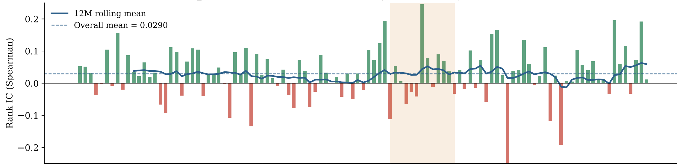
FinBERT_only: Monthly Rank IC (2015-2023) | t-stat = 2.67 | 68% positive months
