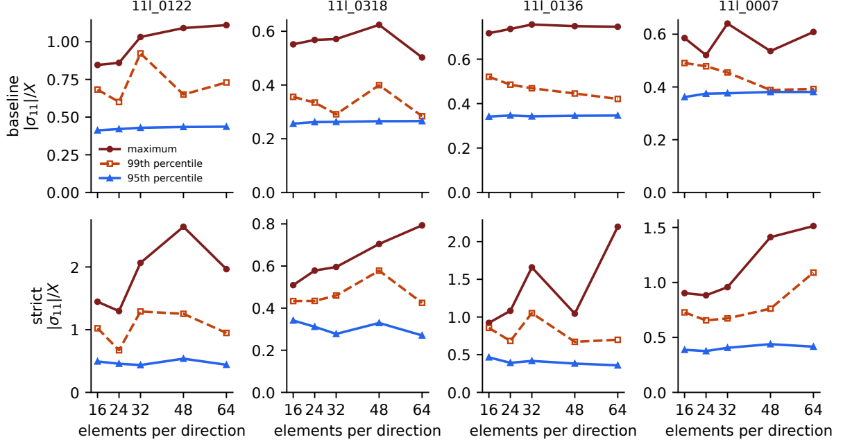
Figure 4: Fiber index against mesh density for four designs, with the DOE coverage law (top) and with plies stopped at their turnaround radius (bottom).
