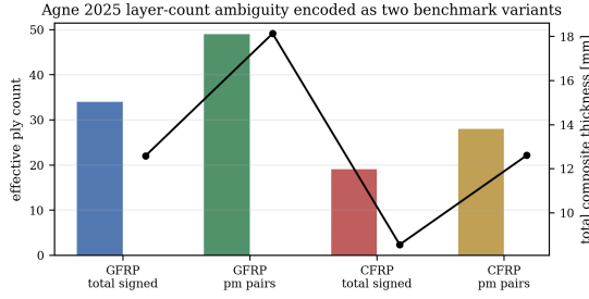
Figure 6: Impact of ply counting interpretations on the total shell thickness for the Agne 2025 benchmark.
