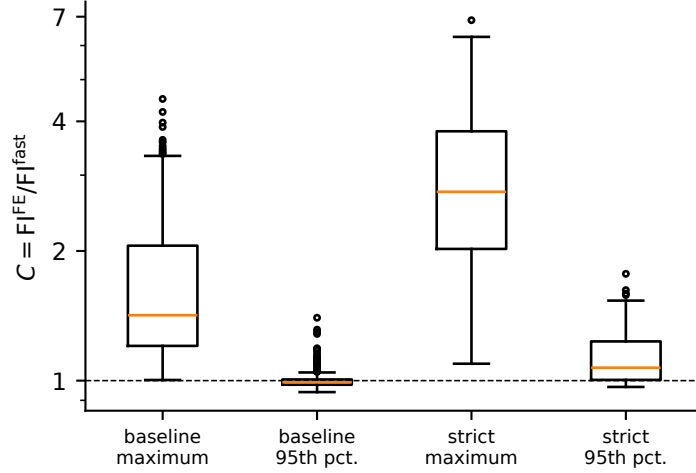
Figure 5: Distribution of the correction factor for four targets (log scale).
