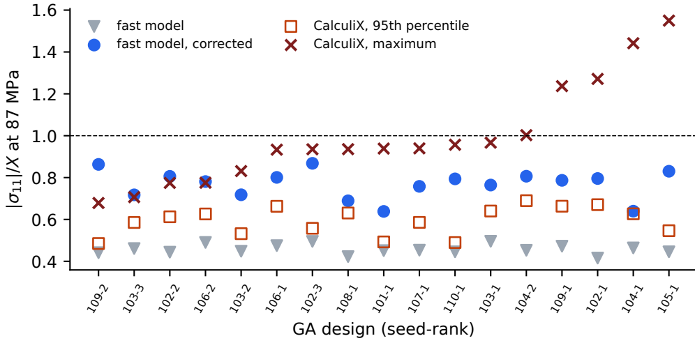
Figure 3: Fiber index of the 17 GA designs at 87 MPa (data/ga_statistical_validation.csv).
