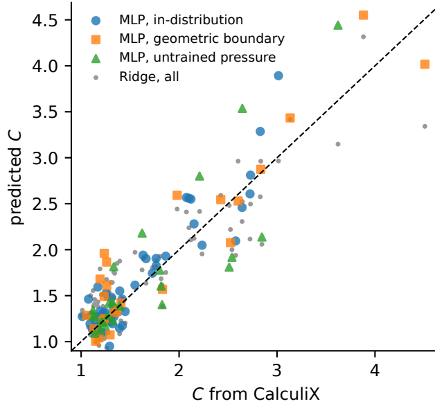
Figure 1: Predicted against CalculiX correction factor on the 96 held-out designs (data/extended_statistical_eval_predictions.csv).
