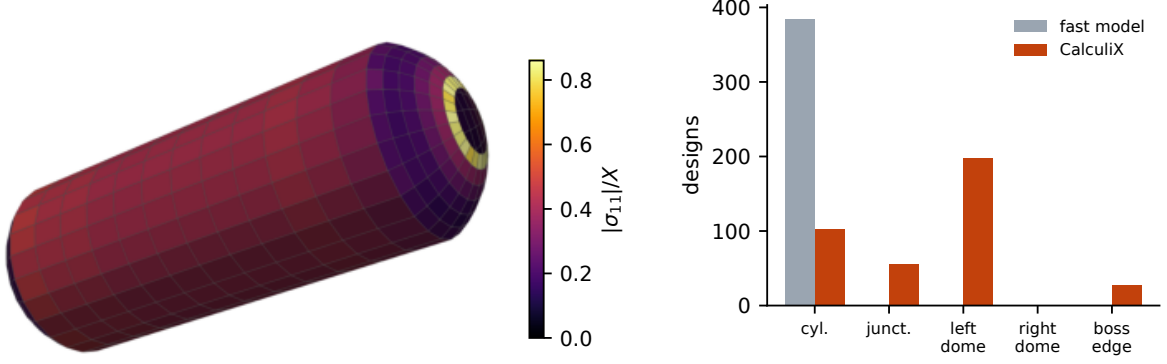
Figure 2: Left: fiber index of design 111_0122 at 70 MPa, worst ply per element. Right: zone of the maximum over the 384 designs for both models.
