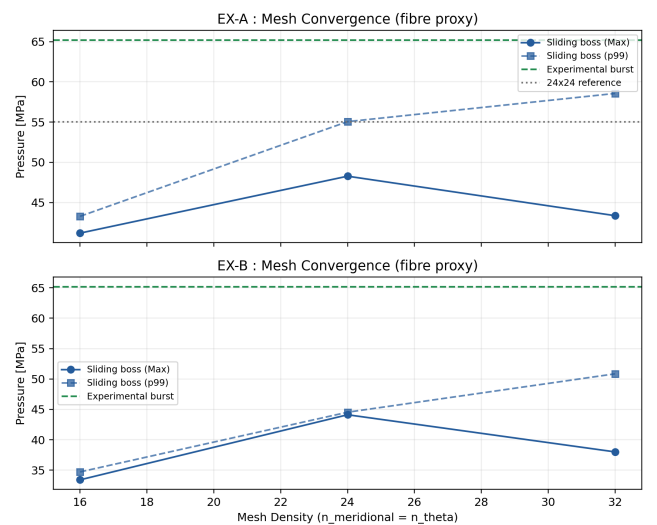
Figure 3: Mesh sensitivity on vessels EX-A and EX-B of Jin et al. [4]. The strict maximum oscillates because of the polar singularities; the p99 quantile increases monotonically but has not converged at 32x32.
