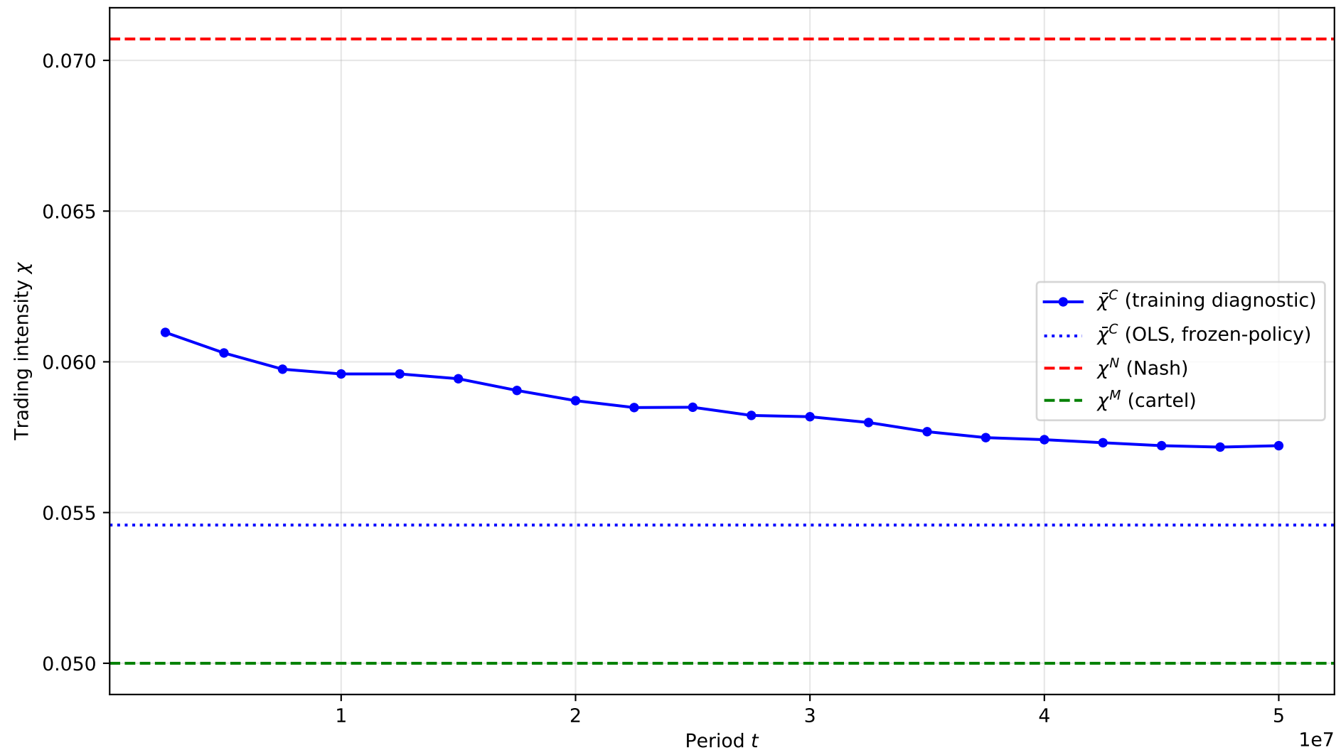
Convergence ( l = 2 , \xi = 0 , method="sequential")
