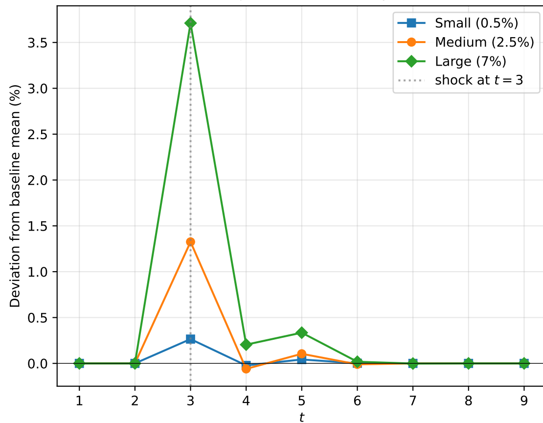
Price IRF ( \xi = 0 , method=sequential)
