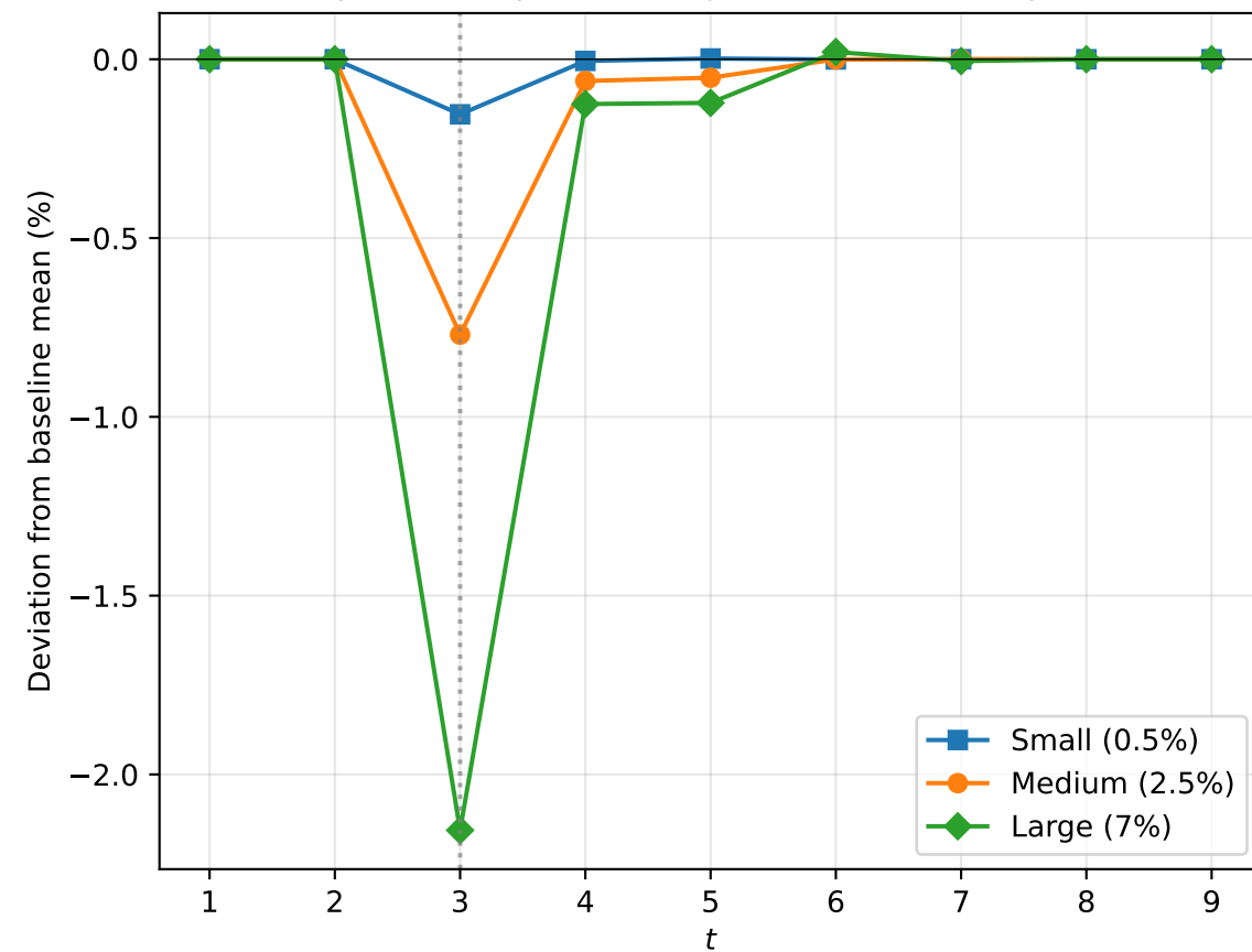
Per-speculator profit IRF ( \xi = 0 , method=sequential)
