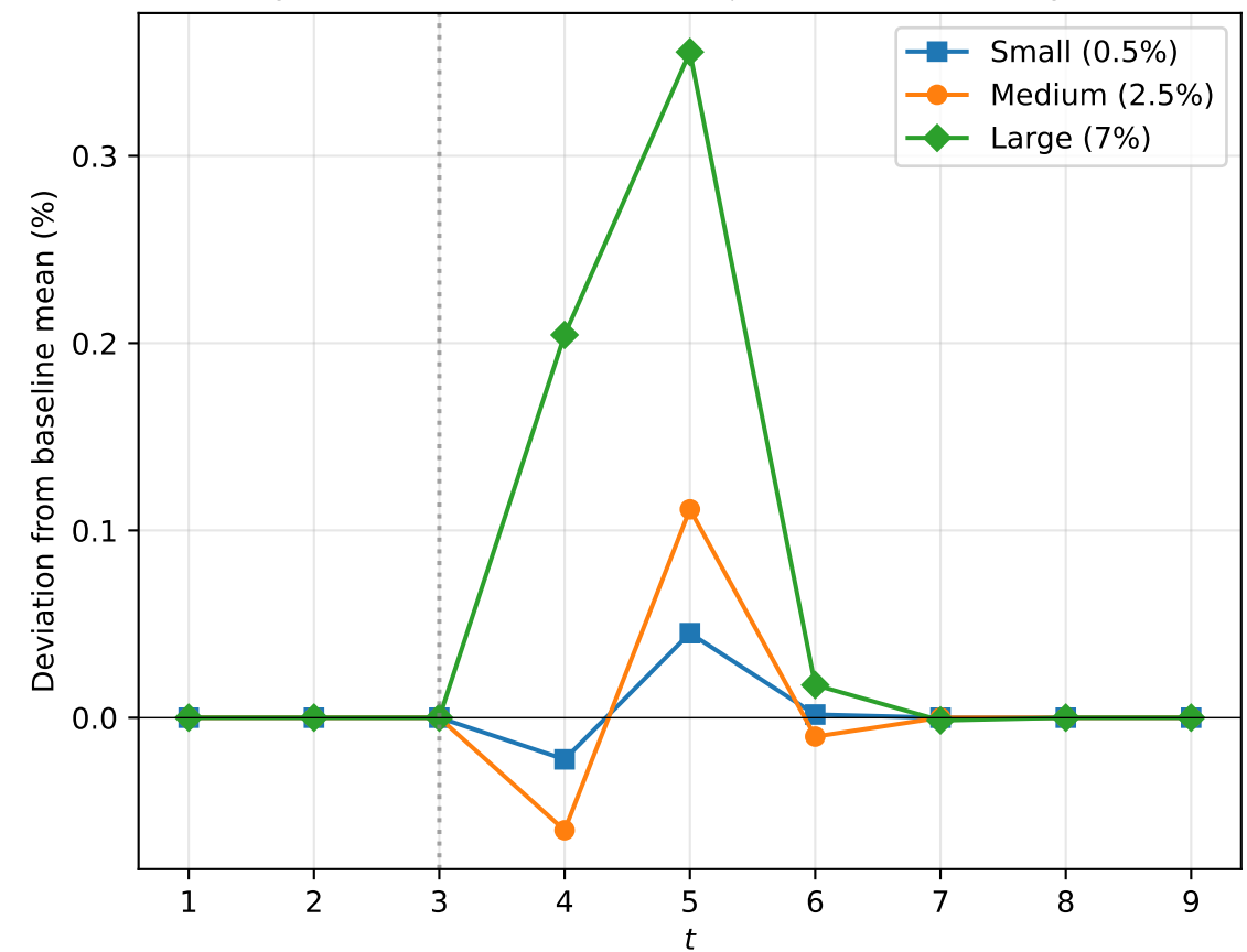
Per-speculator order flow IRF ( \xi = 0 , method=sequential)
