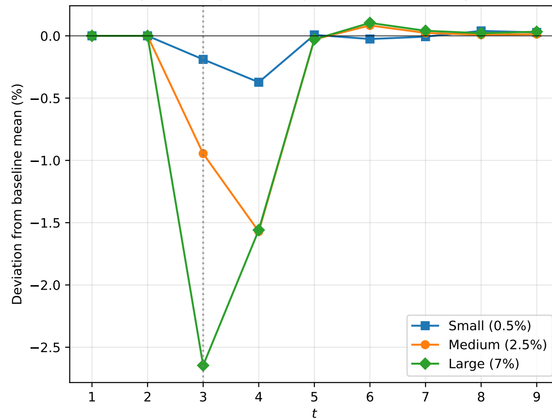
Per-speculator profit IRF ( \xi = 500 , method=sequential)
