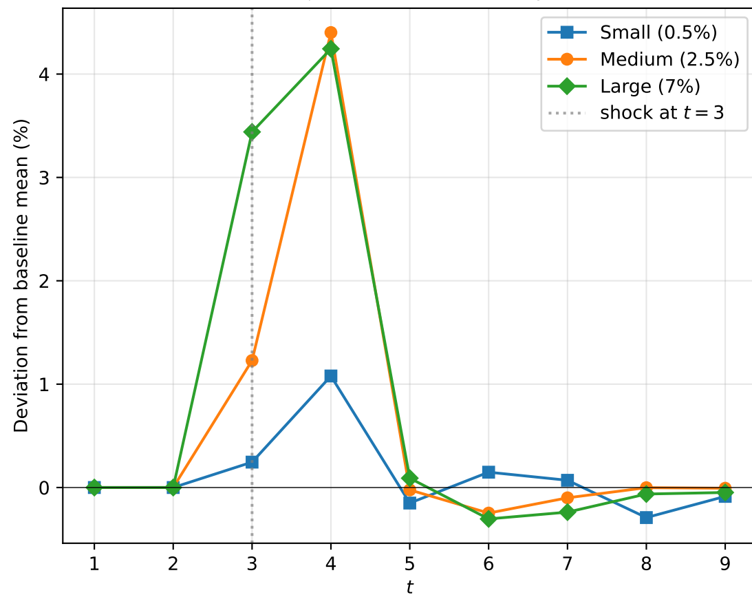
Price IRF ( \xi = 500 , method=sequential)
