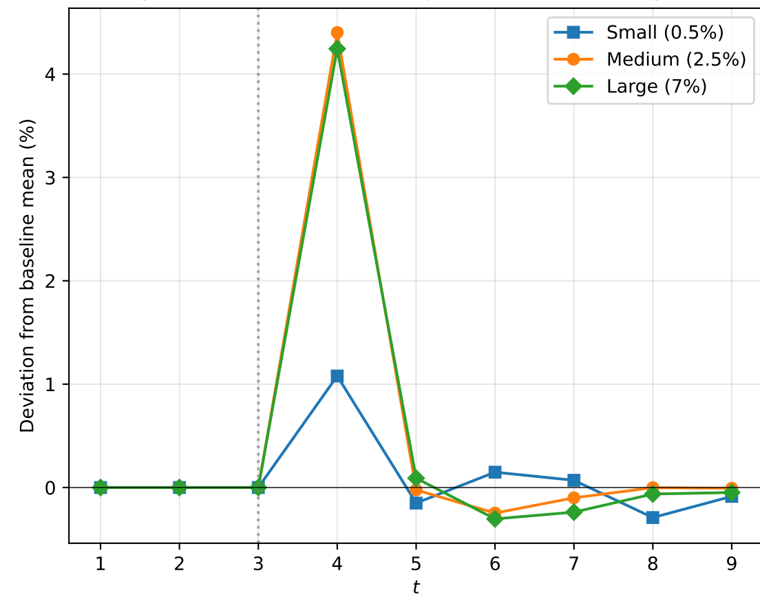
Per-speculator order flow IRF ( \xi = 500 , method=sequential)
