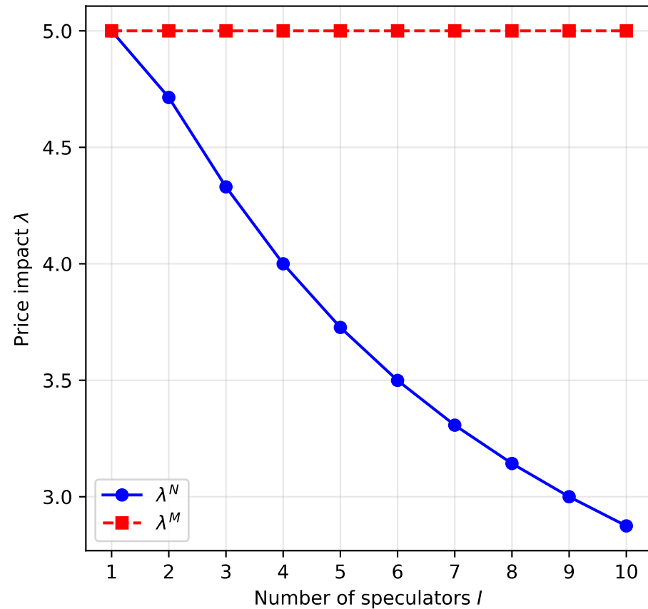
Price Impact \lambda^N and \lambda^M
