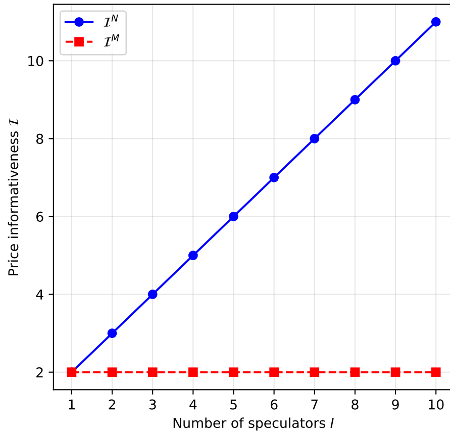
Price Informativeness \mathcal{I}^N and \mathcal{I}^M
