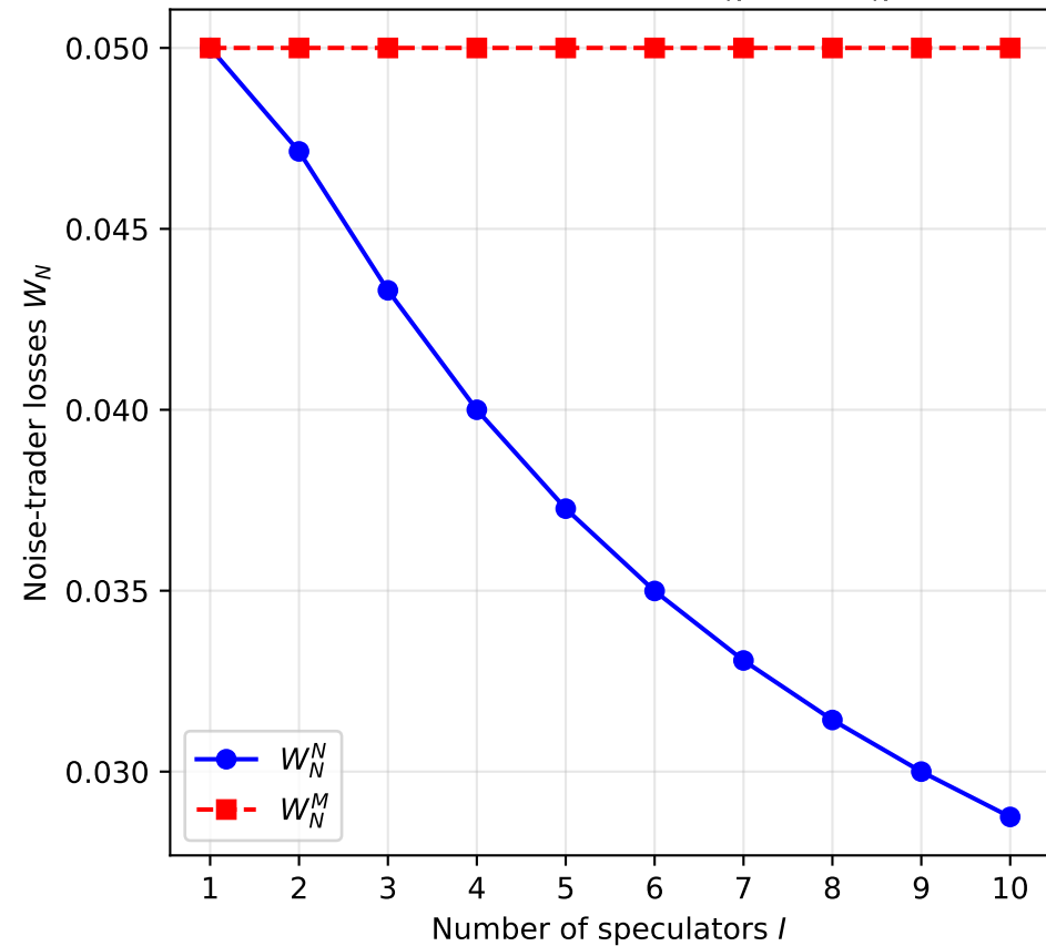
Noise-Trader Losses W_N^N and W_N^M
