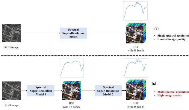
Fig. 1. Previous approach is shown in (a) and our approach is shown in (b). Our approach obtains higher-quality spectral super-resolution results and multiple spectral resolutions by cascading the models in the spectral dimension.
