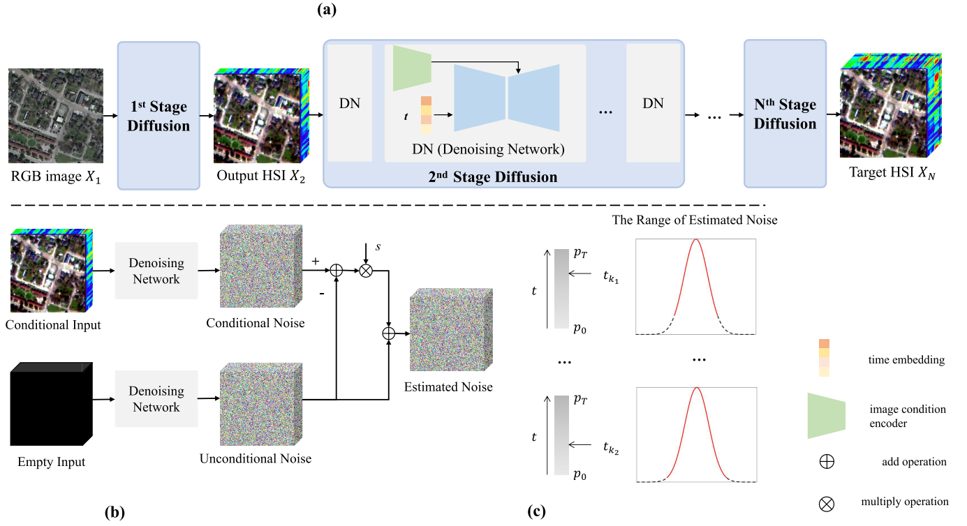
Fig. 2. Overview of the proposed method. (a) Pipeline of SCDM. SCDM consists of a series of conditional diffusion models cascaded in the spectral dimension. The conditional input to the first stage of the diffusion model is the RGB remote sensing images, and the subsequent diffusion models are conditioned on the output of the previous stage. The generation process of each stage starts with noise and iteratively denoises to yield the desired outputs for the corresponding spectral bands. (b) Sampling procedure with ICMG, which achieves better utilization of the input conditions by mixing conditional and unconditional outputs weighted in sampling. (c) Process of PDT, where p represents the truncation percentile. At the early stages of sampling, the p value is relatively small. As the sampling progresses (with decreasing t ), p increases.
