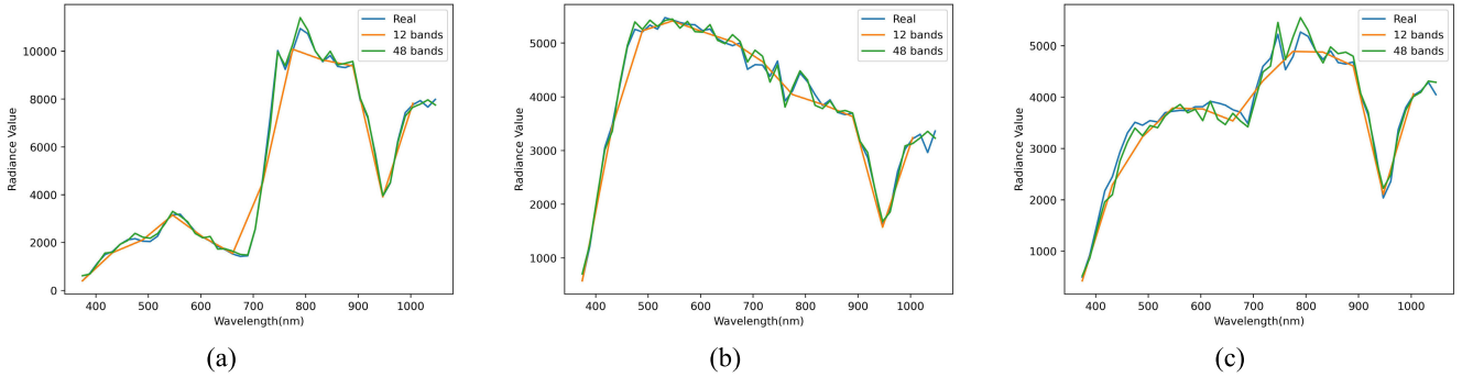
Fig. 7. Comparison between the output and the true value of SCDM for different spectral resolutions. It can be seen that SCDM is a process that goes from coarse to fine in the spectral dimension, and the prediction results are obtained from the gradual refinement of the spectral trend. (a) Grass. (b) Road. (c) Soil.
