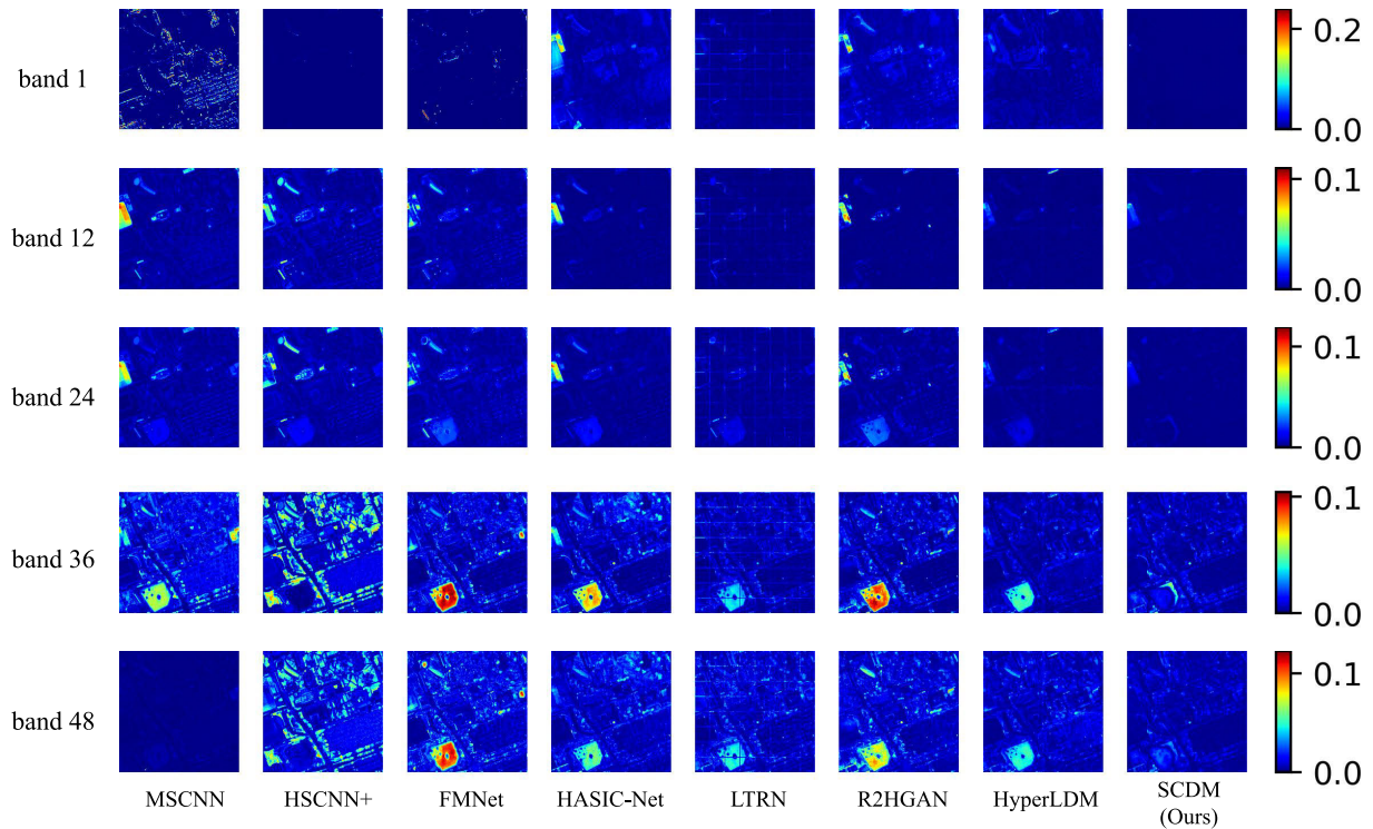
Fig. 4. Absolute differences between the reconstructed images and the ground truth at bands 1, 12, 24, 36, and 48 on the IEEE grss_dfc_2018 dataset. The scale values on the color bar on the right side represent the absolute difference divided by the maximum possible value in the reconstructed HSI.
