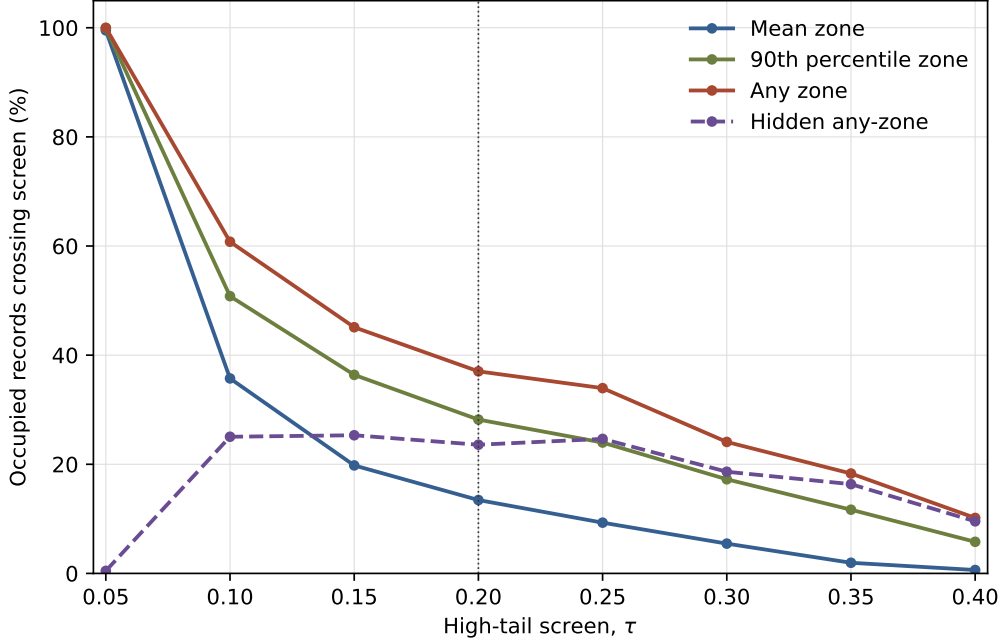
Figure 4: Sensitivity of high-tail exceedance to the selected p_{\text{tail}} screen. The vertical line marks the manuscript reporting screen \tau = 0.20 . The persistent gap between mean-zone, p90-zone, and any-zone exceedance shows that the zone-aggregation result is not specific to a single threshold.
