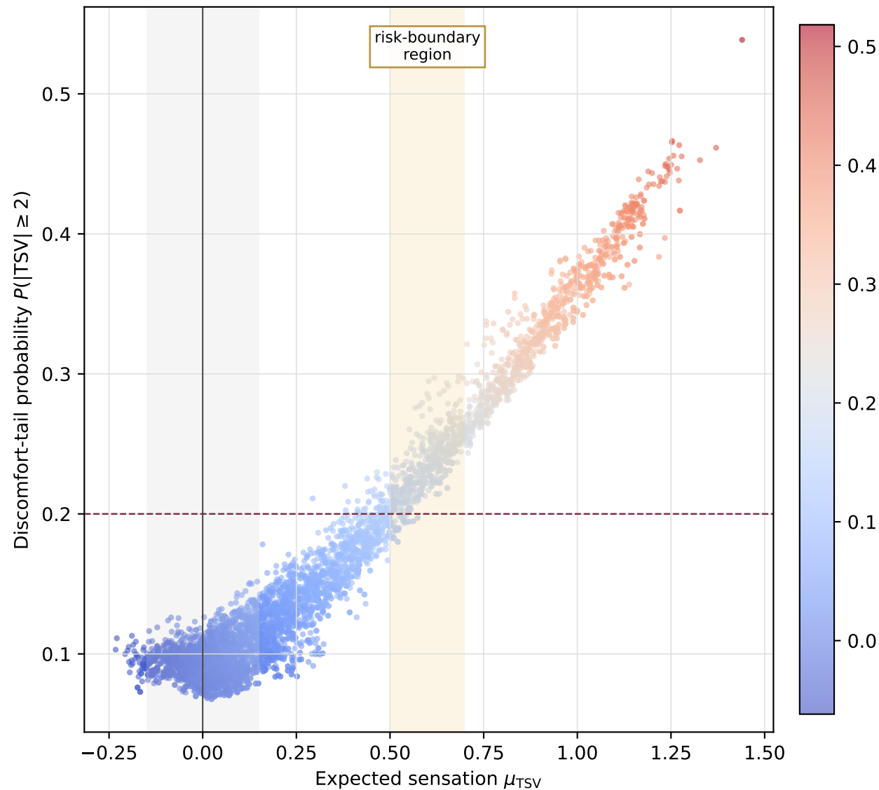
A. Expected sensation is informative but not sufficient near the diagnostic boundary
