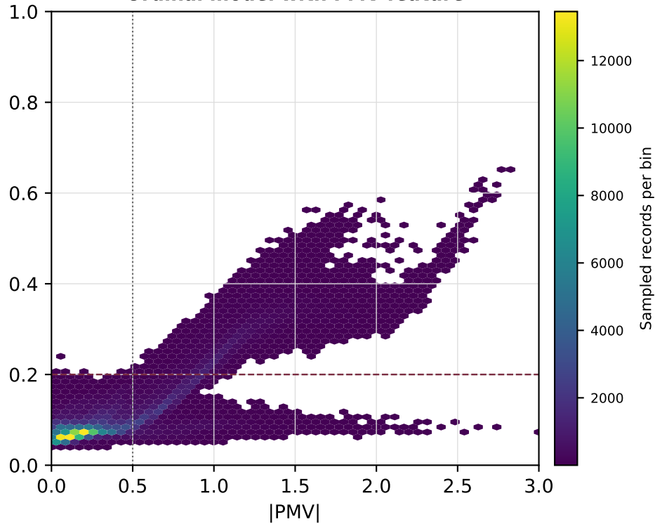
Ordinal model with PMV feature
