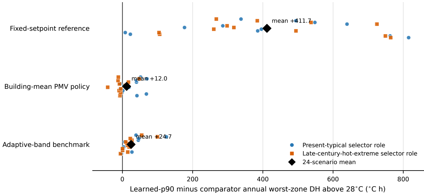
Primary annual thermal comparison on one common horizontal scale
