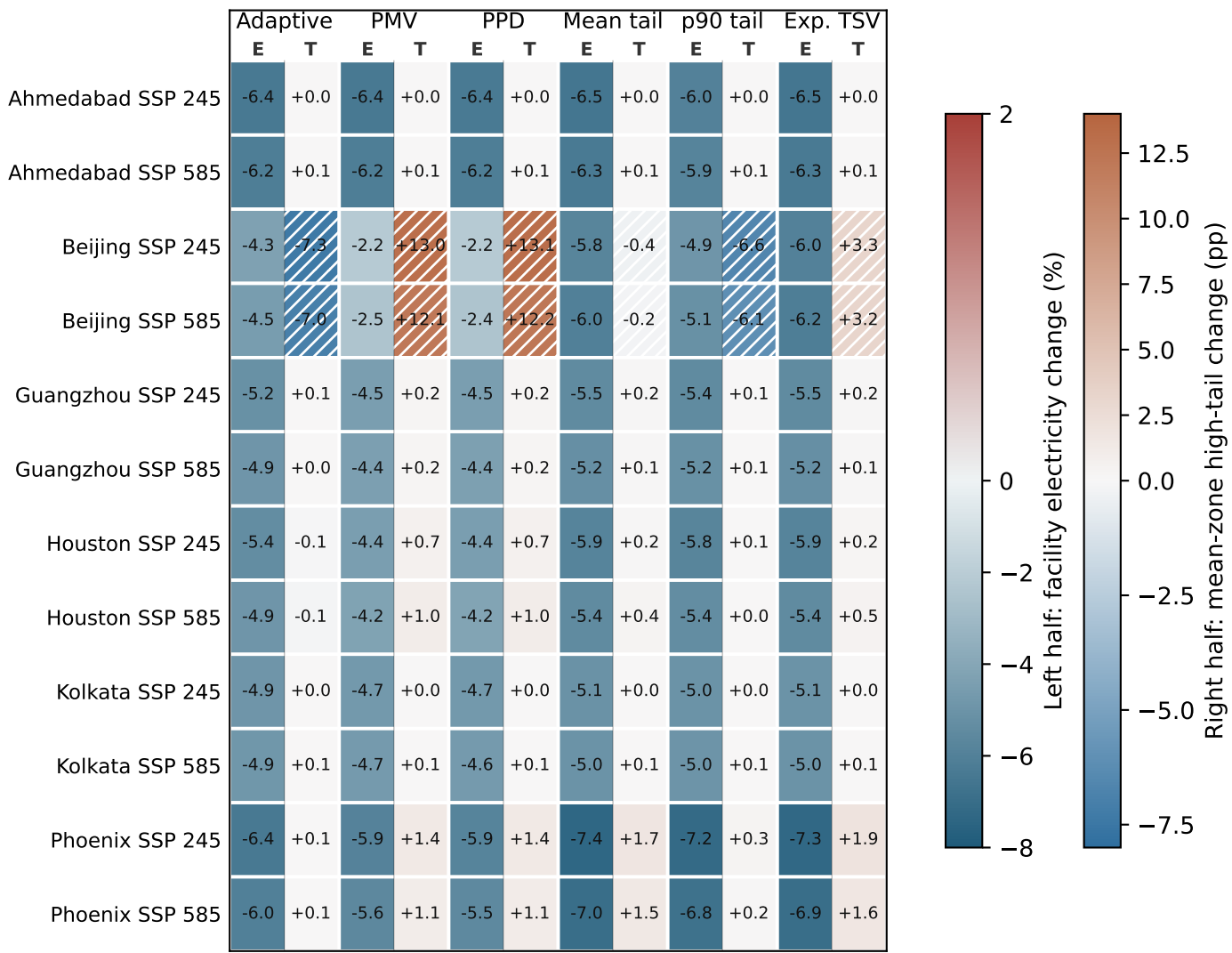
Annual energy-risk matrix: savings, mean tail change, and any-zone hatch
