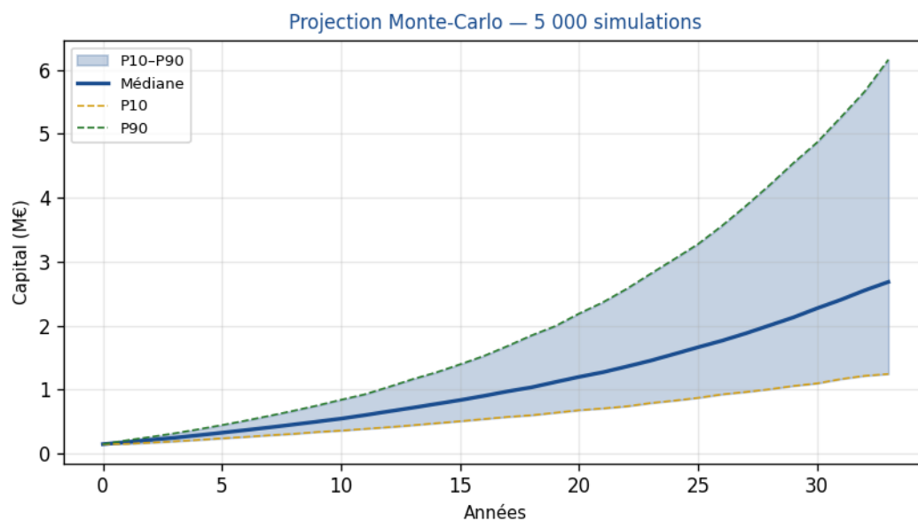
Figure 2 — Projection Monte-Carlo (5 000 simulations)
