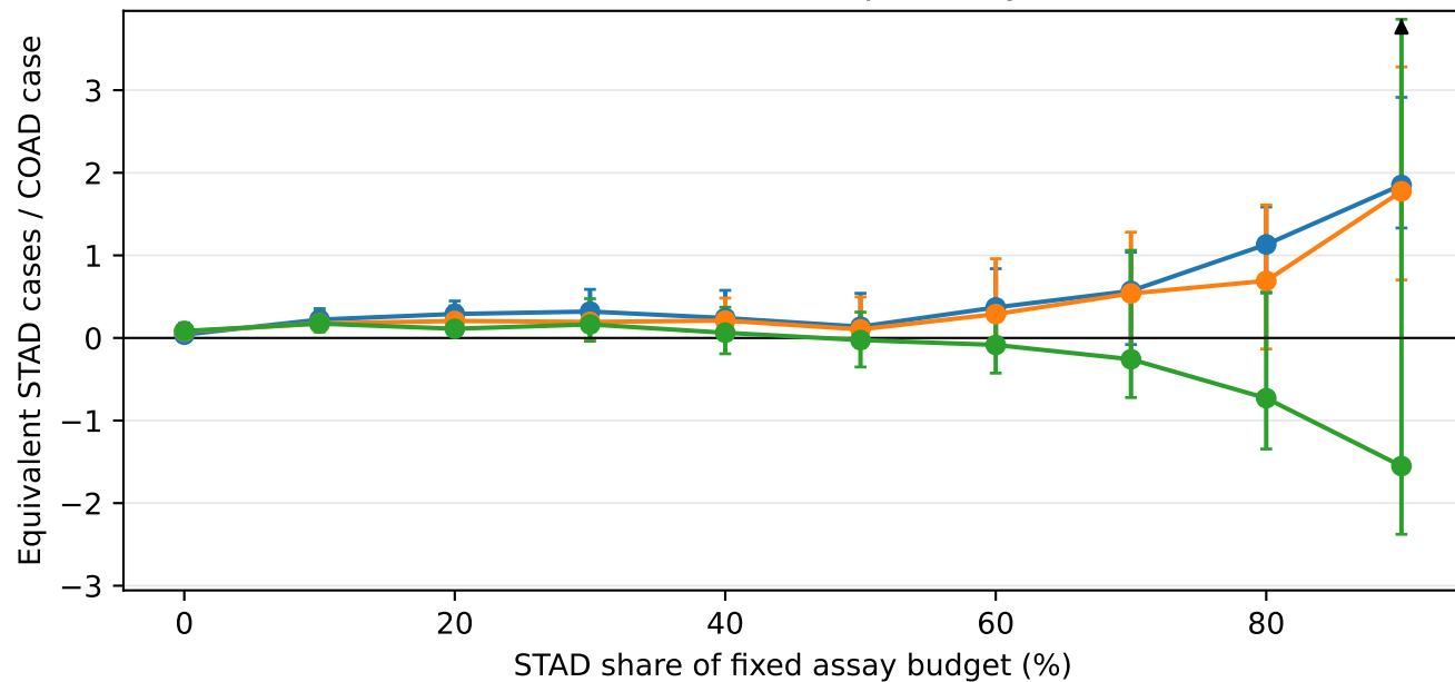
COAD → STAD (exploratory)
