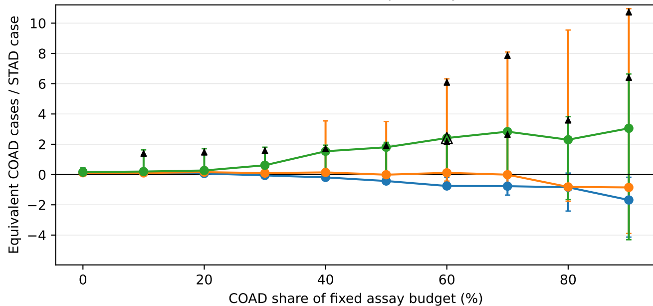
STAD → COAD (exploratory)
