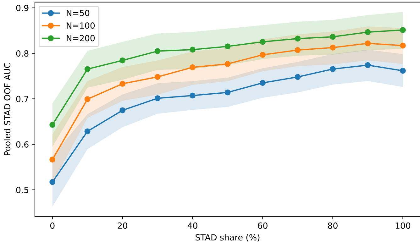
Budget-matched COAD→STAD swap (EXPLORATORY)
