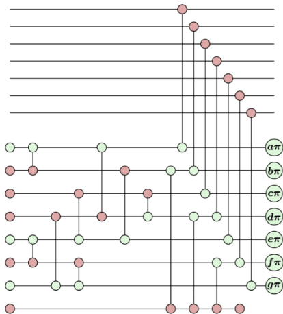
(a) Steane-Style syndrome extraction
