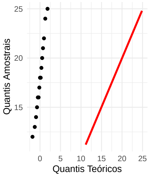
Q-Q Plot Normal
