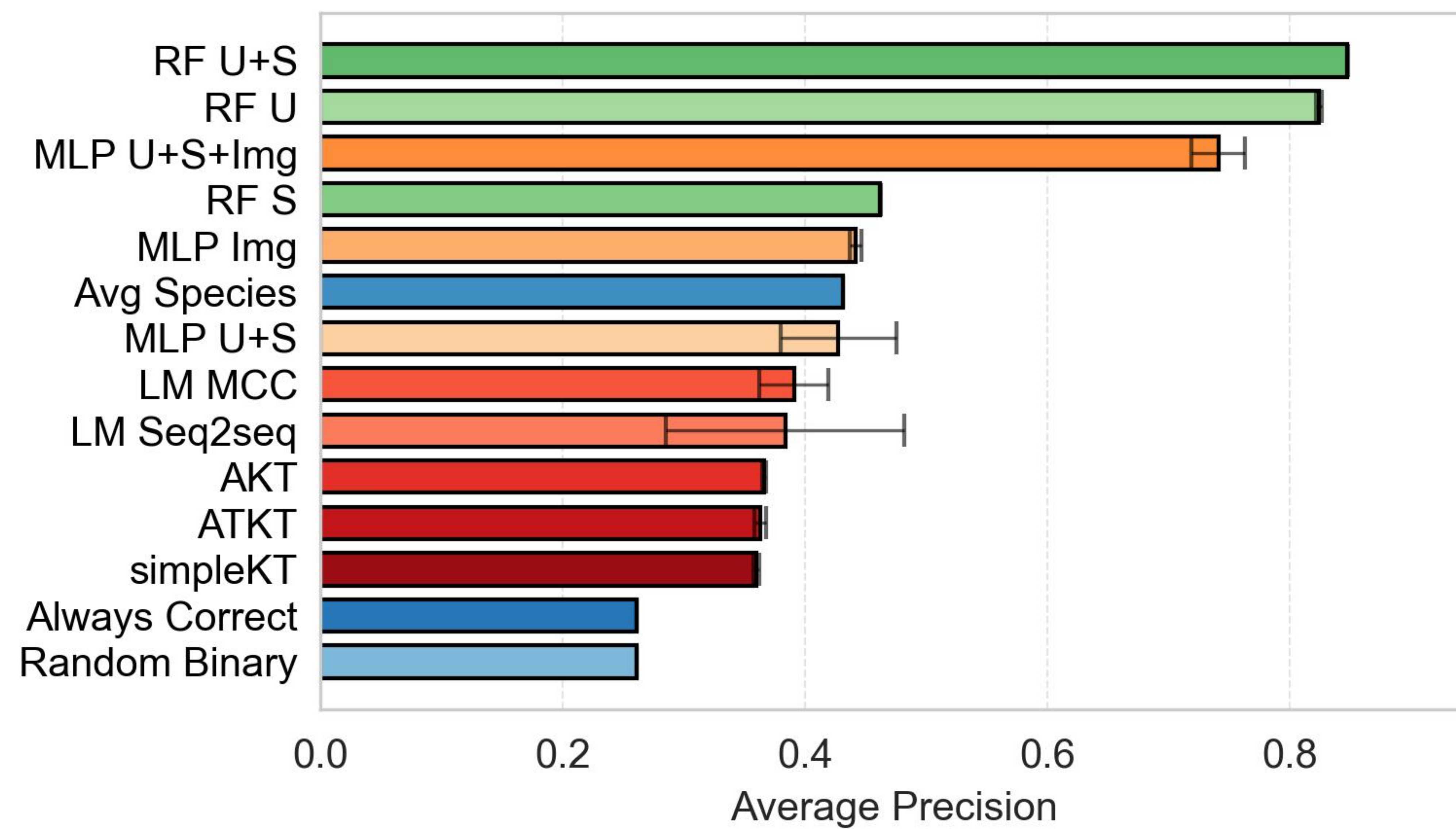
Binary AP - Correctly Predicting User Mistakes
