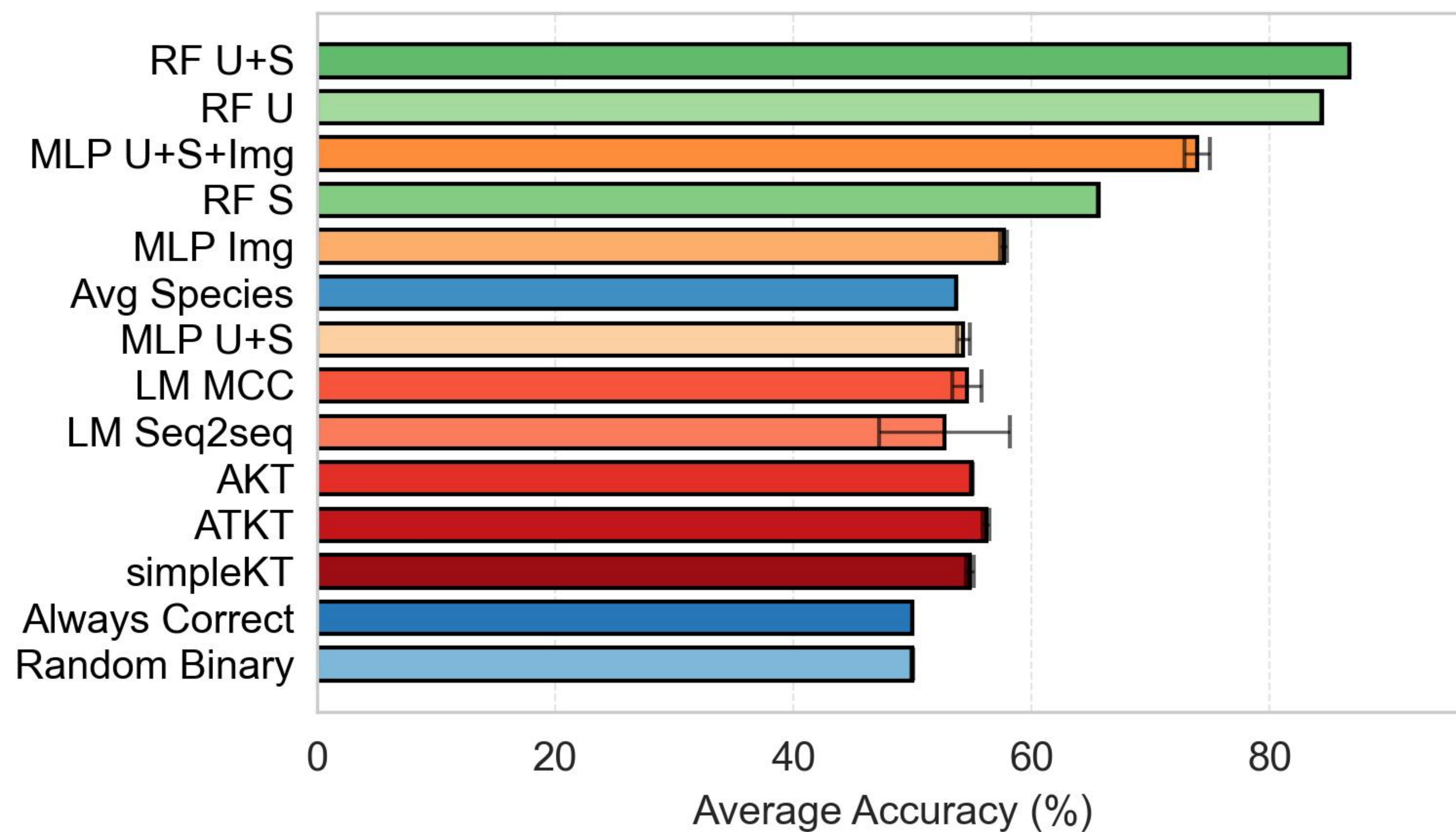
Binary Macro Accuracy
