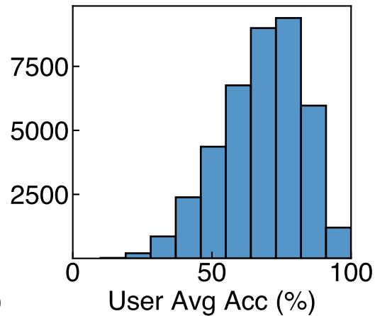
Distribution of User Accuracy
