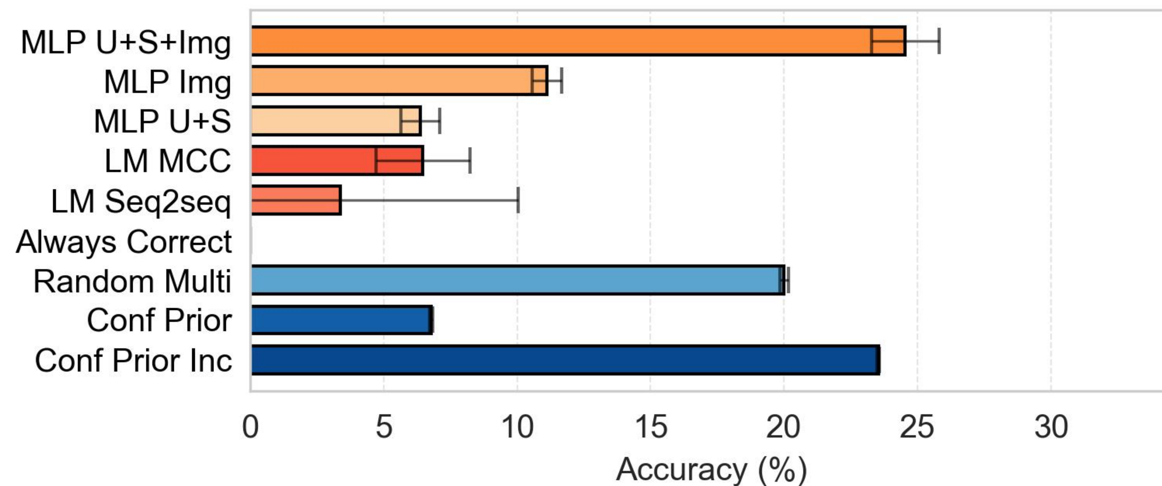
Binary AP - Correctly Predicting User Mistakes
