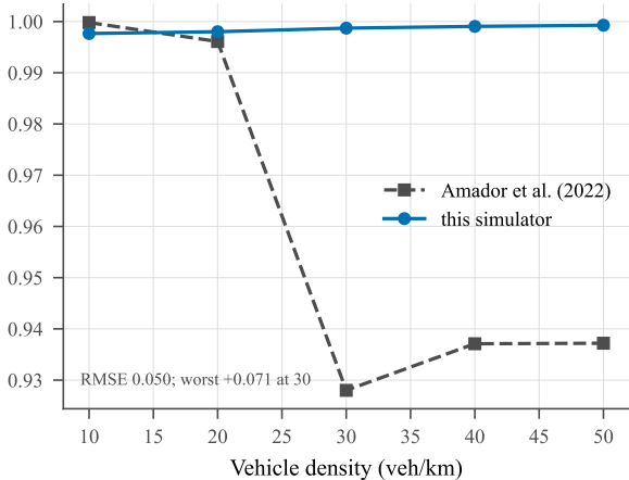
Packet delivery ratio
