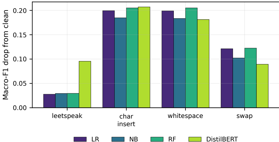
Degradation under character-level attacks
