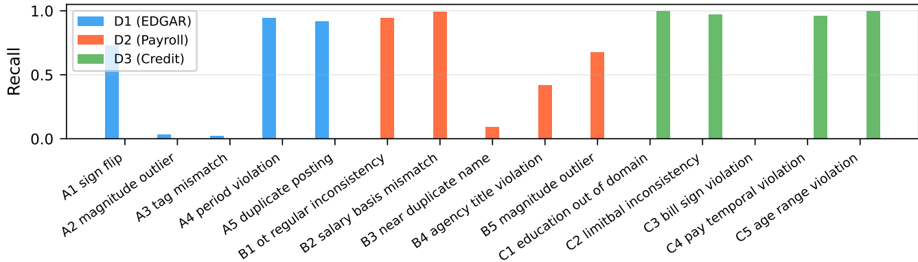
Per-anomaly-family Recall (Hybrid-LR)
