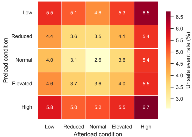
Proposed: unsafe rate over preload-afterload grid
