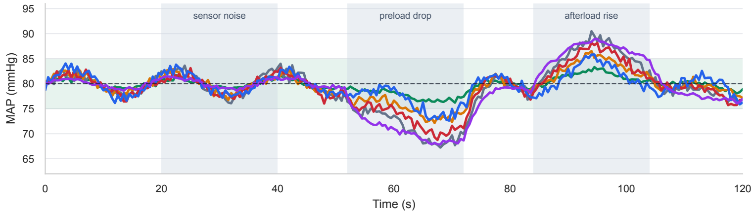
Target MAP versus actual MAP under composite disturbances
