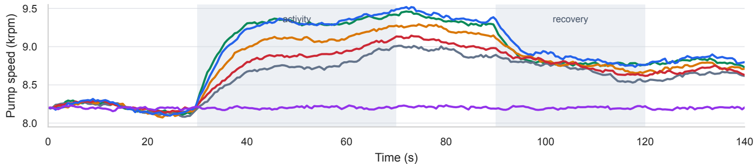
Adaptive pump speed command
