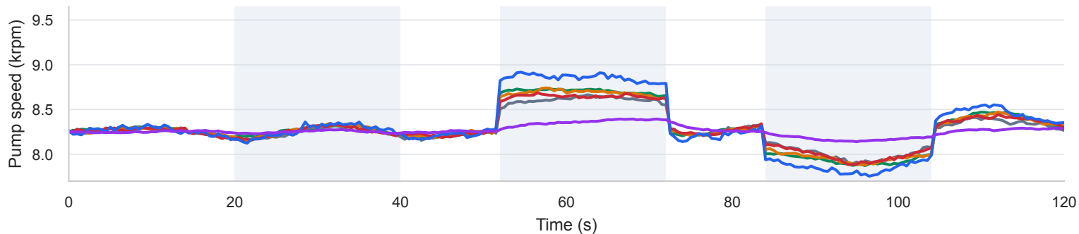
Pump speed command
