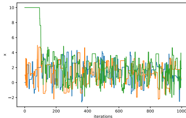
Figure 5: Trace plot
