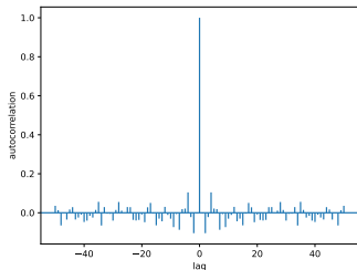
Figure 6: Bon autocorrélogramme
