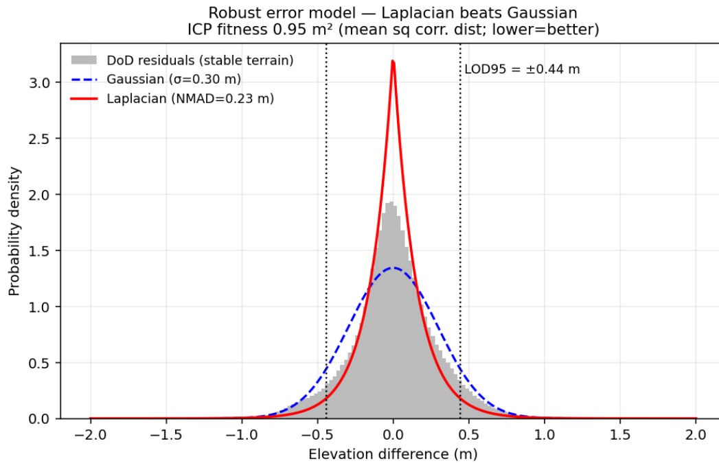
Figure 4. Stable-terrain DoD residuals are sharply Laplacian , not Gaussian — the fat tails would inflate a \sigma -based LOD. This reproduces Barlow's NMAD/Laplacian finding and is the launch point for the proposed per-pixel calibrated-uncertainty layer (O3).
