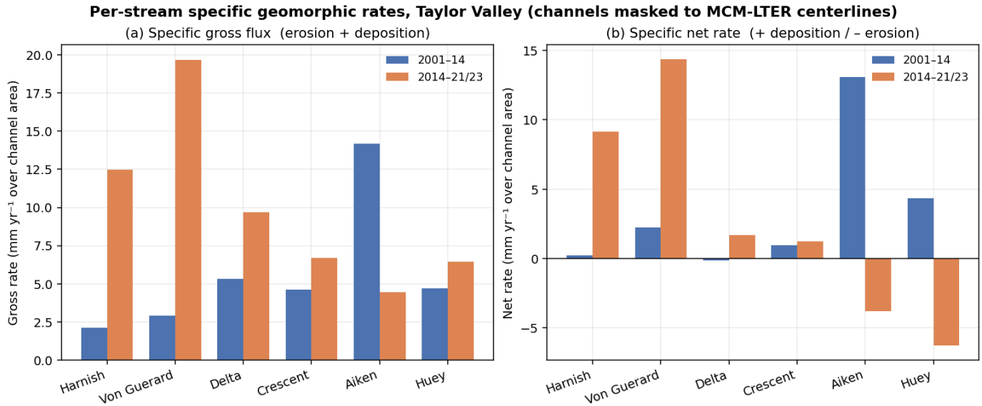
Figure 3. Per-stream rates for six gauged Taylor Valley streams, reported as mm/yr over the channel area rather than raw volume. Gross is total activity (erosion plus deposition); net is the balance (positive = building up, negative = wearing down). Area-normalizing matters because the two epochs don't cover identical footprints (the 2001 lidar swath is narrower), so raw volumes would mix real change with coverage differences.
