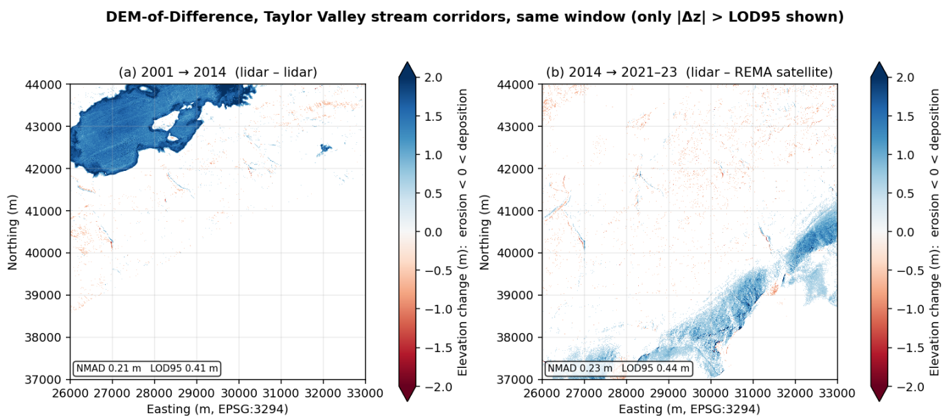
Figure 2. DoD maps over the same Taylor Valley stream-corridor window, showing only changes above the noise floor. Left: 2001→2014 (lidar vs lidar). Right: 2014→2021-23 (lidar vs REMA). Red is erosion, blue is deposition. The big flat patch on the left is Lake Fryxell rising \sim 1.5 m, real change, but water, so an automated screen detects flat water surfaces and drops them from every stream rate.
