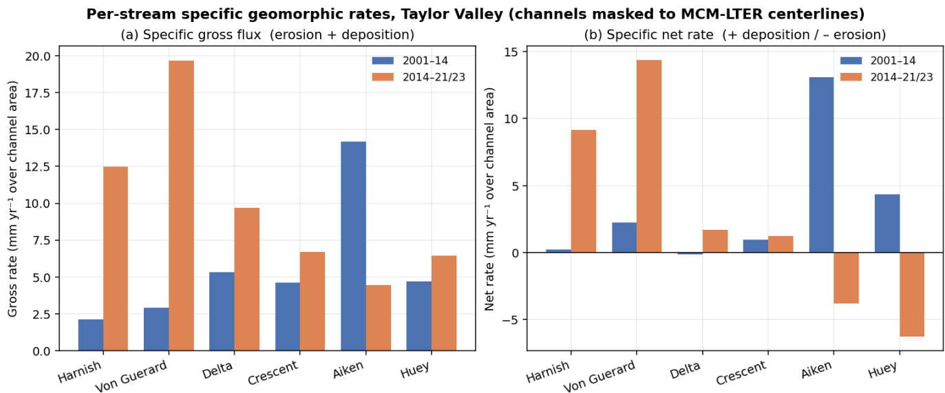
Figure 3. How much sediment each of six gauged Taylor Valley streams moved, per year, in each period. Rates are reported per square meter of channel (mm/yr of surface change) rather than as raw m 3 /yr totals: the surveys do not all cover the same footprint (the 2001 lidar swath is narrower than the satellite coverage), and a per-area rate cannot be inflated simply because one survey saw more ground.
