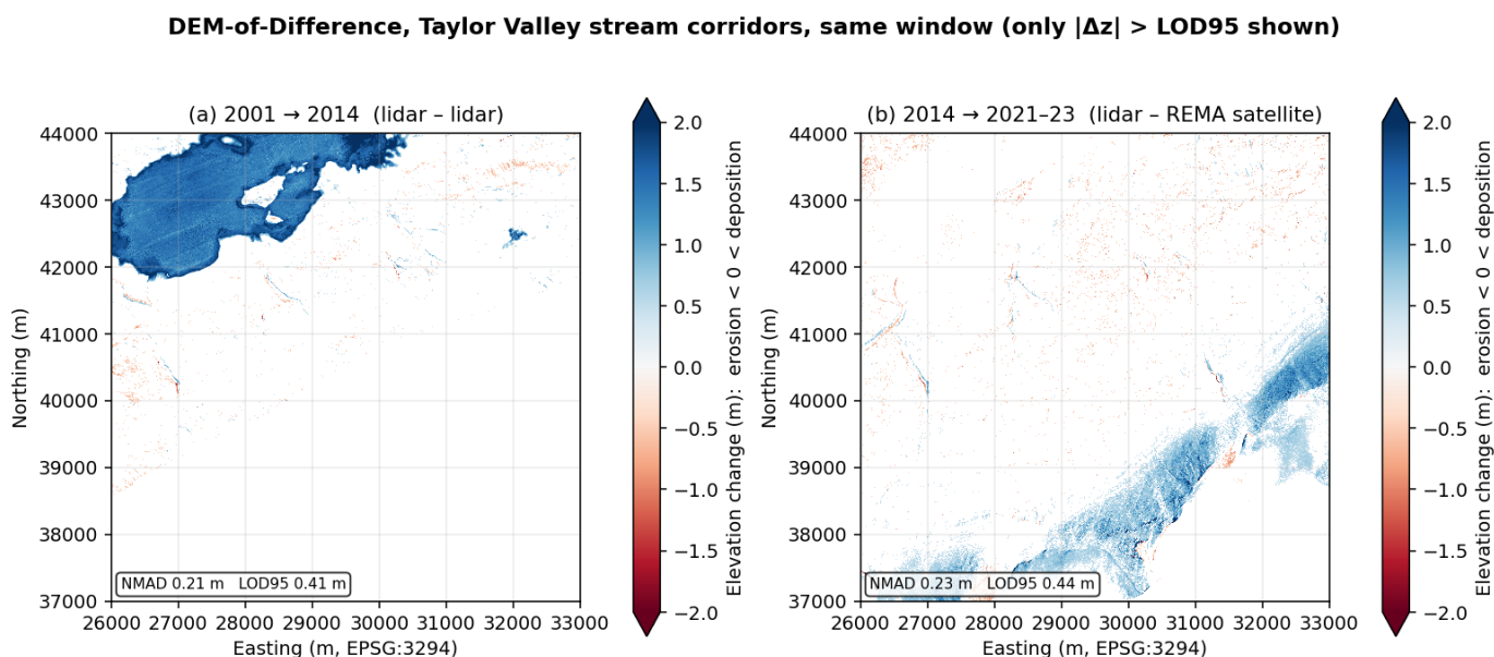
Figure 2. Elevation change over the same Taylor Valley stream-corridor window in two periods: (a) 2001→2014, comparing two lidar surveys; (b) 2014→2021-23, comparing lidar against the REMA satellite DEM. Red = surface lowered (erosion), blue = surface raised (deposition). Pixels are drawn only where the change exceeds the detection floor (LOD95) — i.e., is too large to be measurement noise — and coherent erosion/deposition patterns emerge above that floor. The broad flat patch in (a) is not sediment at all:
