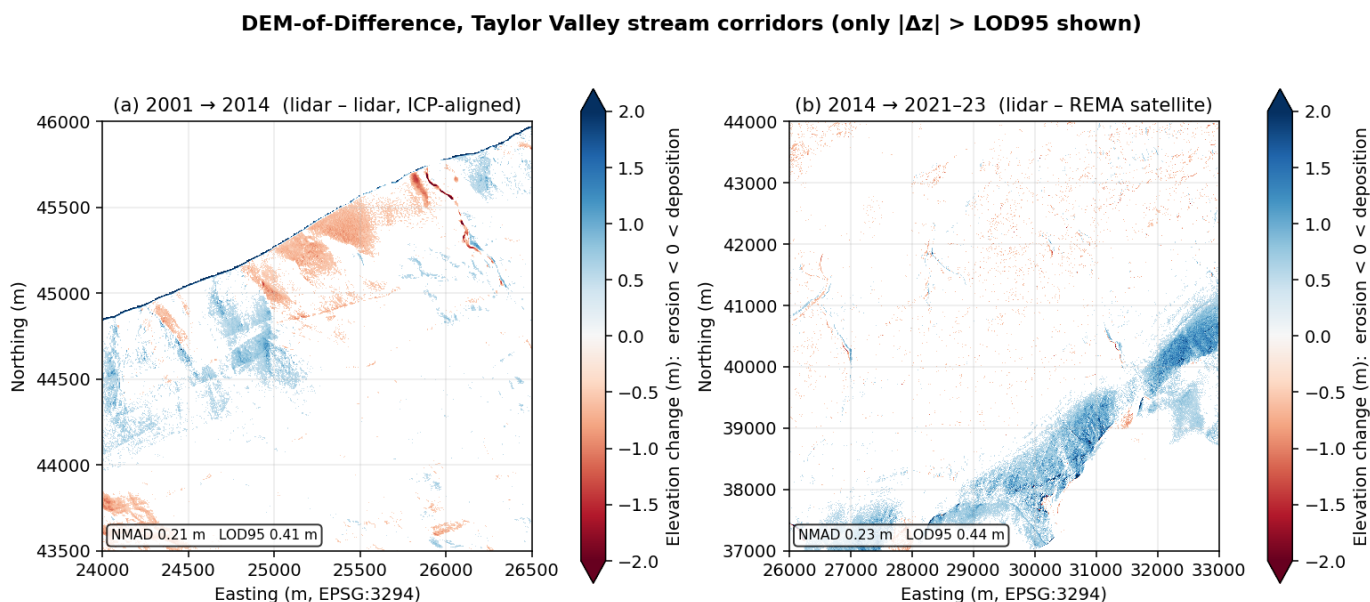
Figure 2. DEM-of-Difference, Taylor Valley stream corridors, only |\Delta z| > \text{LOD95} shown. (a) 2001→2014 lidar-lidar, ICP-aligned; (b) 2014→2021-23 lidar-REMA. Coherent erosion/deposition patterns emerge above the noise floor; REMA auto-reprojected from EPSG:3031 to the lidar grid.
