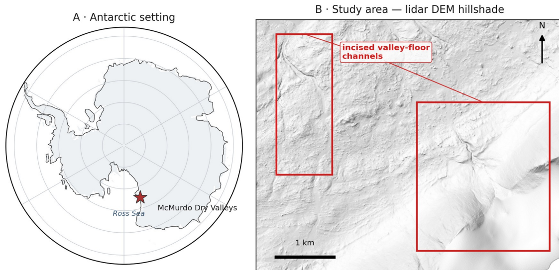
Figure 1. Study area. (A) The McMurdo Dry Valleys within Antarctica (coastline: Natural Earth). (B) Hillshade of the study-area lidar DEM (1 m), showing the incised valley-floor channels this project measures;
