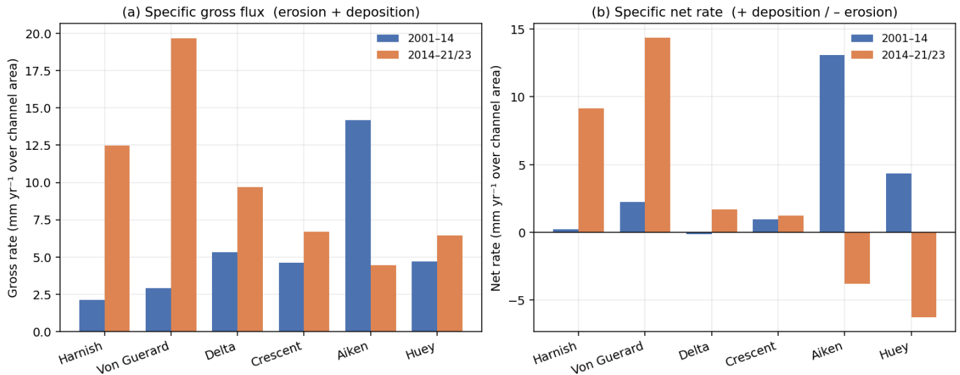
Figure 3. Per-stream specific (area-normalized, mm/yr) gross and net sediment-flux rates for six gauged Taylor Valley streams, both epochs, channels masked to MCM-LTER centerlines. Specific rates are used because the valid-data footprint differs between epochs (the 2001 ATM lidar swath is narrower than REMA coverage), so raw m^3/yr totals would confound real change with coverage.
