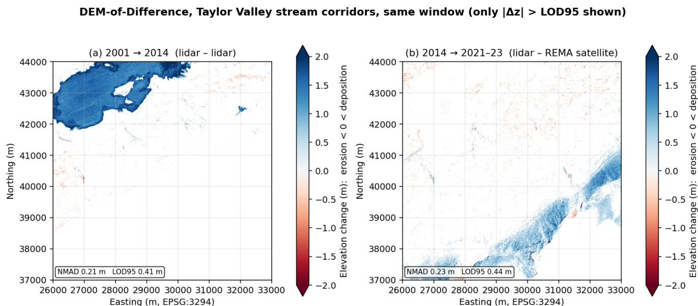
Figure 2. *DEM-of-Difference over the same Taylor Valley stream-corridor window, only
