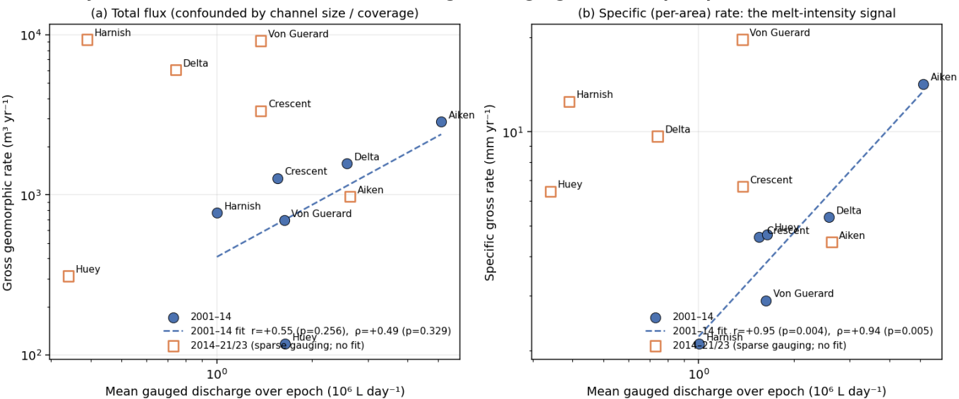
Figure 5. Per-stream geomorphic rate vs. mean gauged melt discharge (log-log; lake-level signal screened out). In the lidar-lidar epoch the specific (area-normalized) rate scales strongly with discharge: Pearson r = +0.95 ( p = 0.004 ), Spearman \rho = +0.94 ( p = 0.005 ), and the relationship survives leaving out any single stream. The REMA epoch shows no coherent relation under sparse post-2015 gauge coverage (48–362 gauged days per stream) and is plotted without a fit. This motivates O1 directly: where gauges are dense the melt-sediment link is strong, so the proposed work will replace patchy gauging with modeled melt energy (PDD/insolation/active-layer) to extend attribution across epochs and valleys, turning correlation into attribution.
