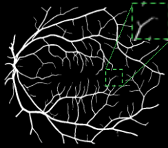
SA-UNet
