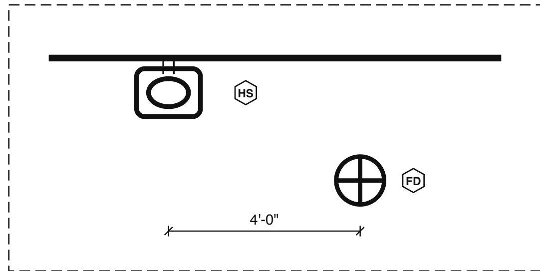
2 HAND SINK STATION · TYP. OF 4 SCALE: 1/2" = 1'-0"
