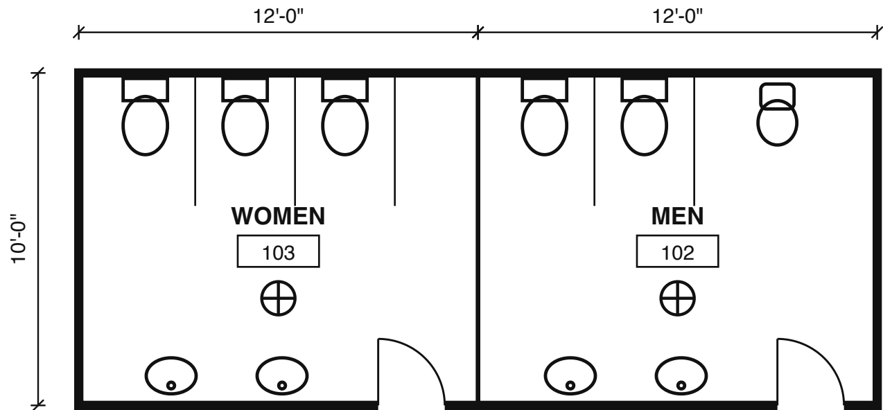
1 ENLARGED RESTROOM PLAN SCALE: 1/4" = 1'-0"
