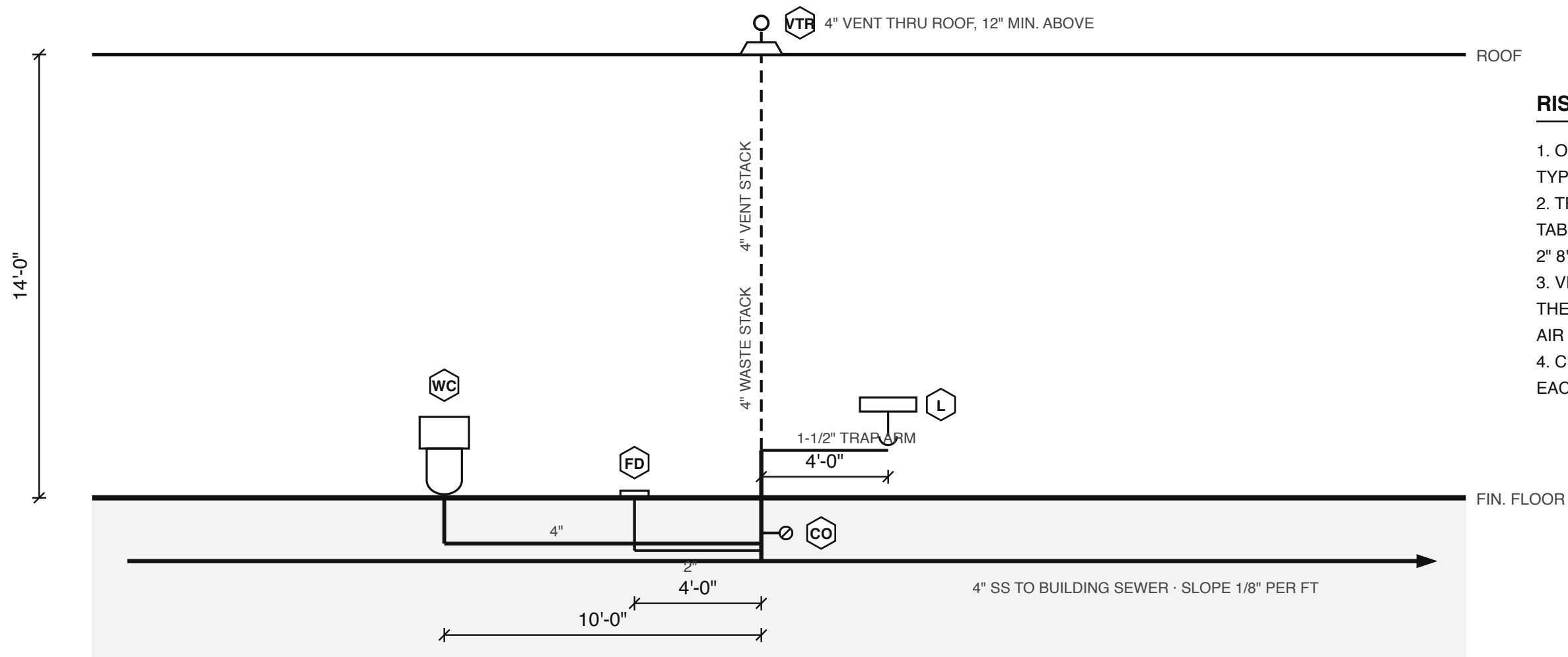
1 WASTE & VENT RISER, RESTROOMS 102 / 103, TYP. SCALE: 1/4" = 1'-0"
