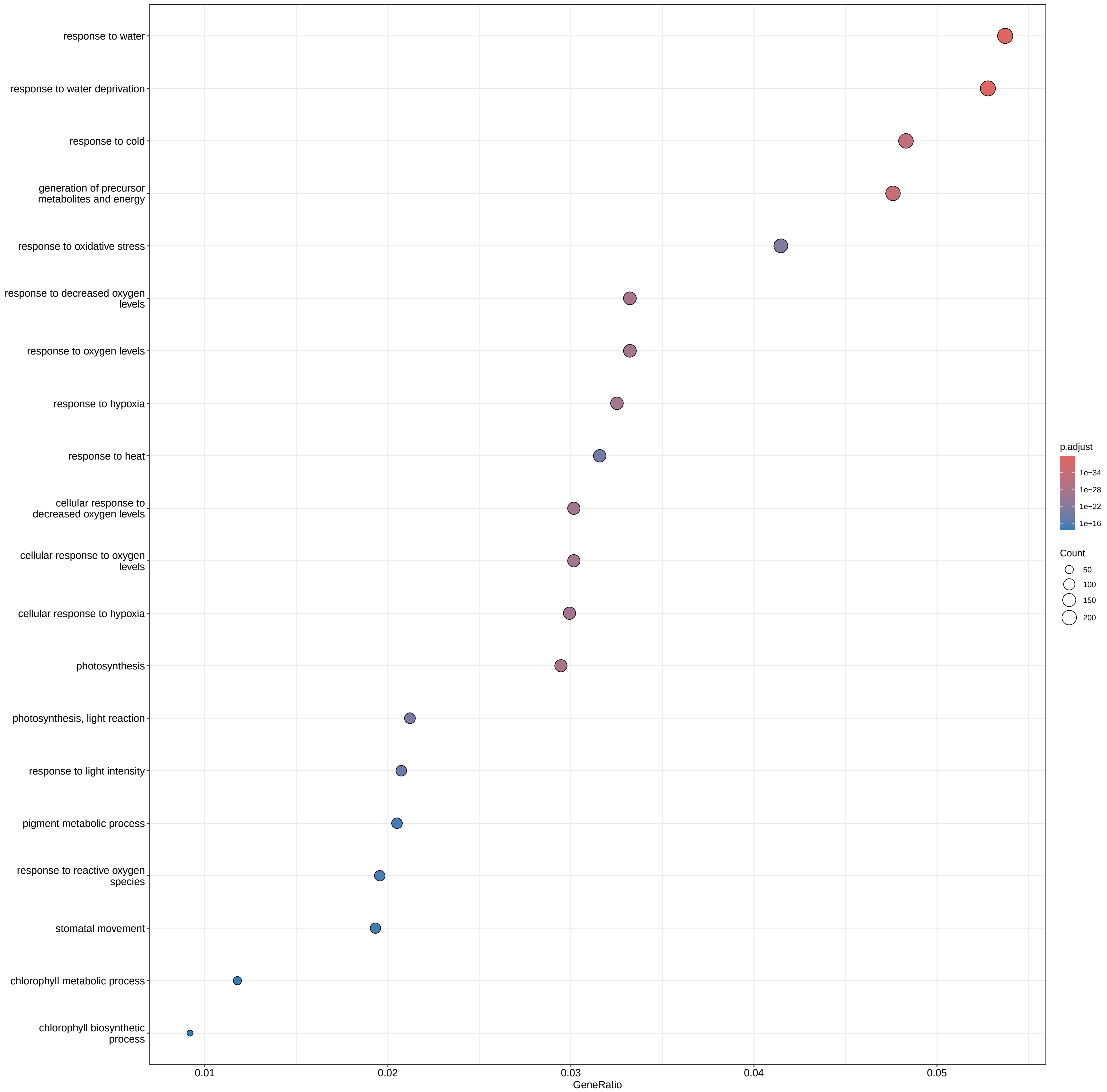
GO Enrichment – Mesophyll_WT_vs_pifq
