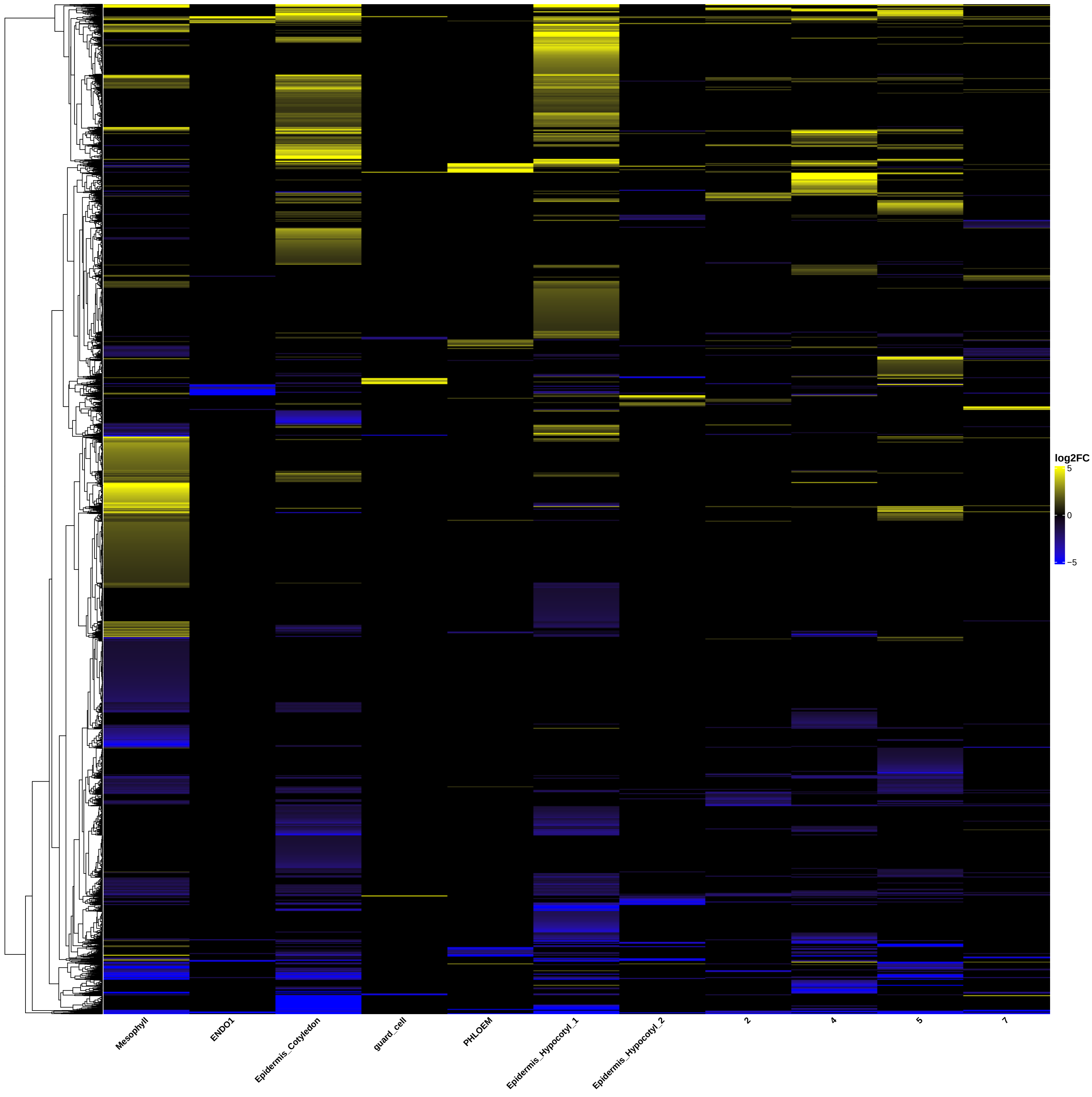
log2FC - WT_vs_pifq (8461 genes)
