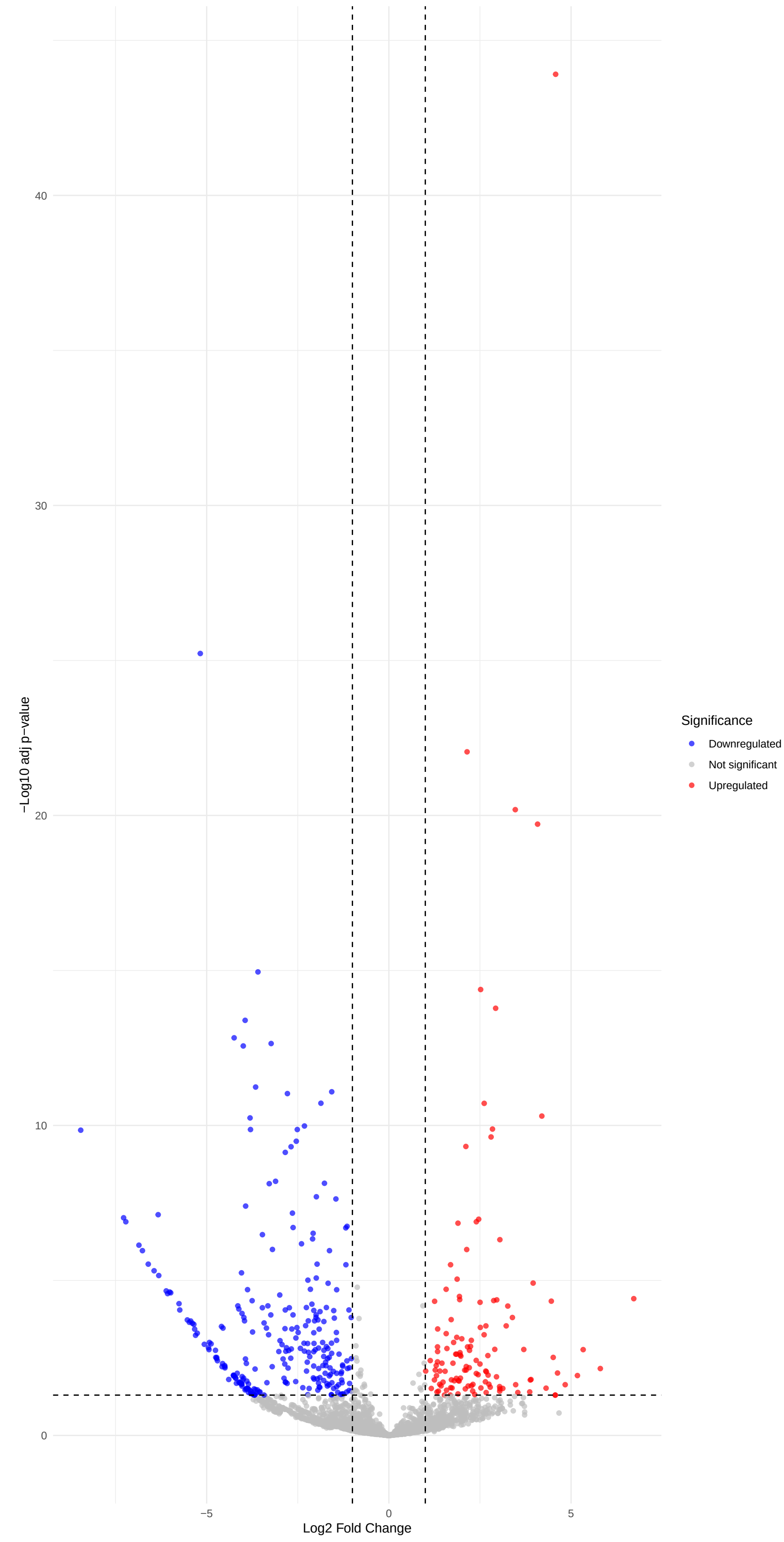
Volcano Plot: Epidermis_Hypocotyl_2_WT_vs_pifq
