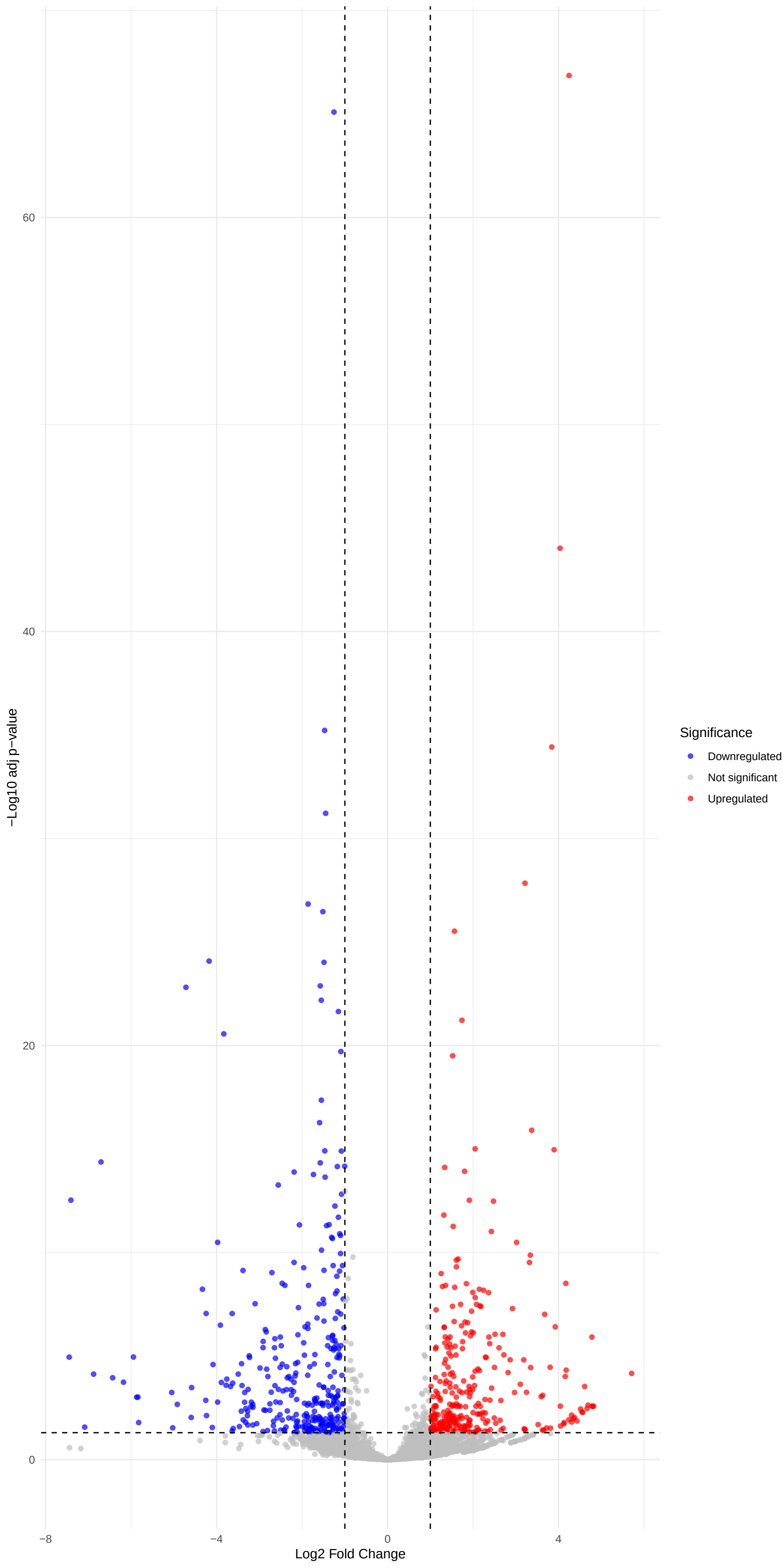
Volcano Plot: 2_WT_vs_pifq
