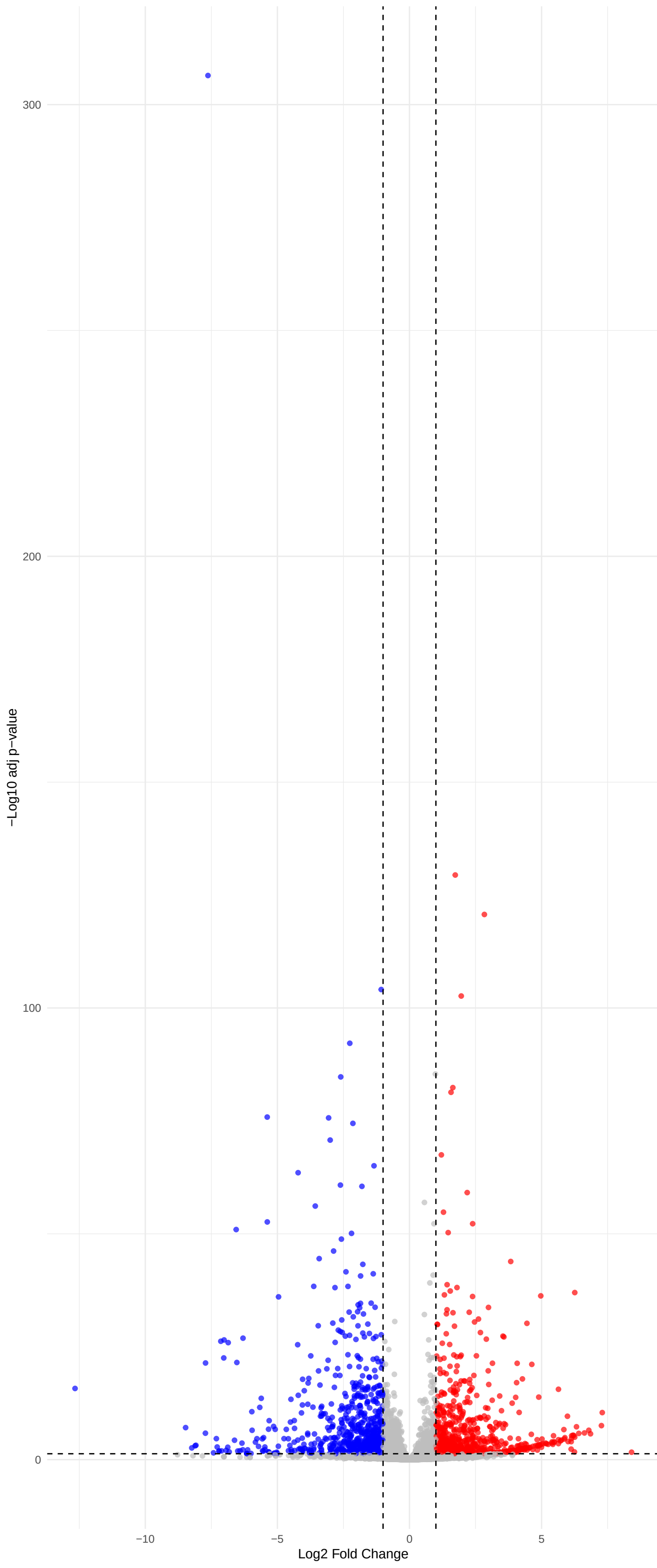
Volcano Plot: 5_WT_vs_pifq
