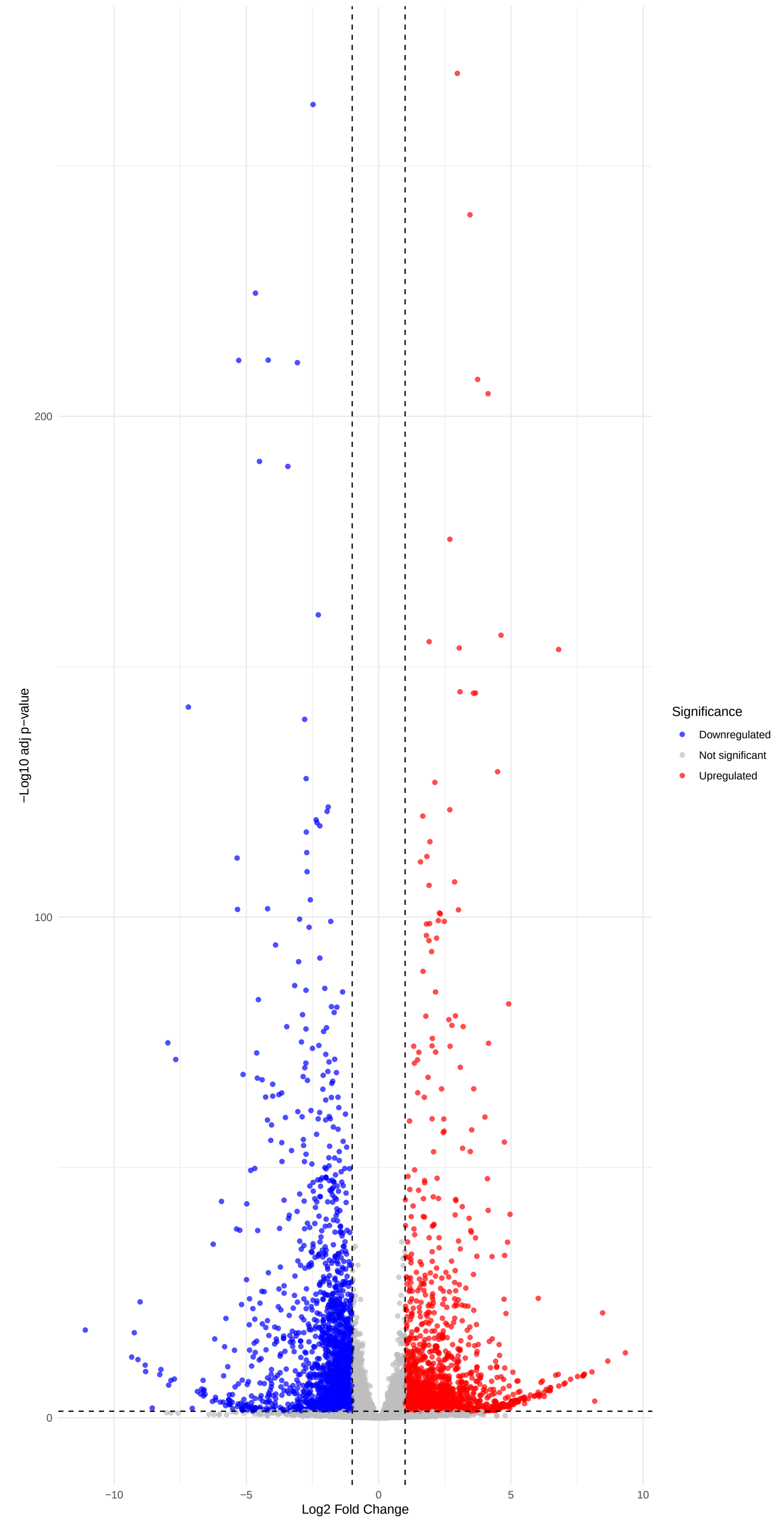
Volcano Plot: Mesophyll_WT_vs_pifq
