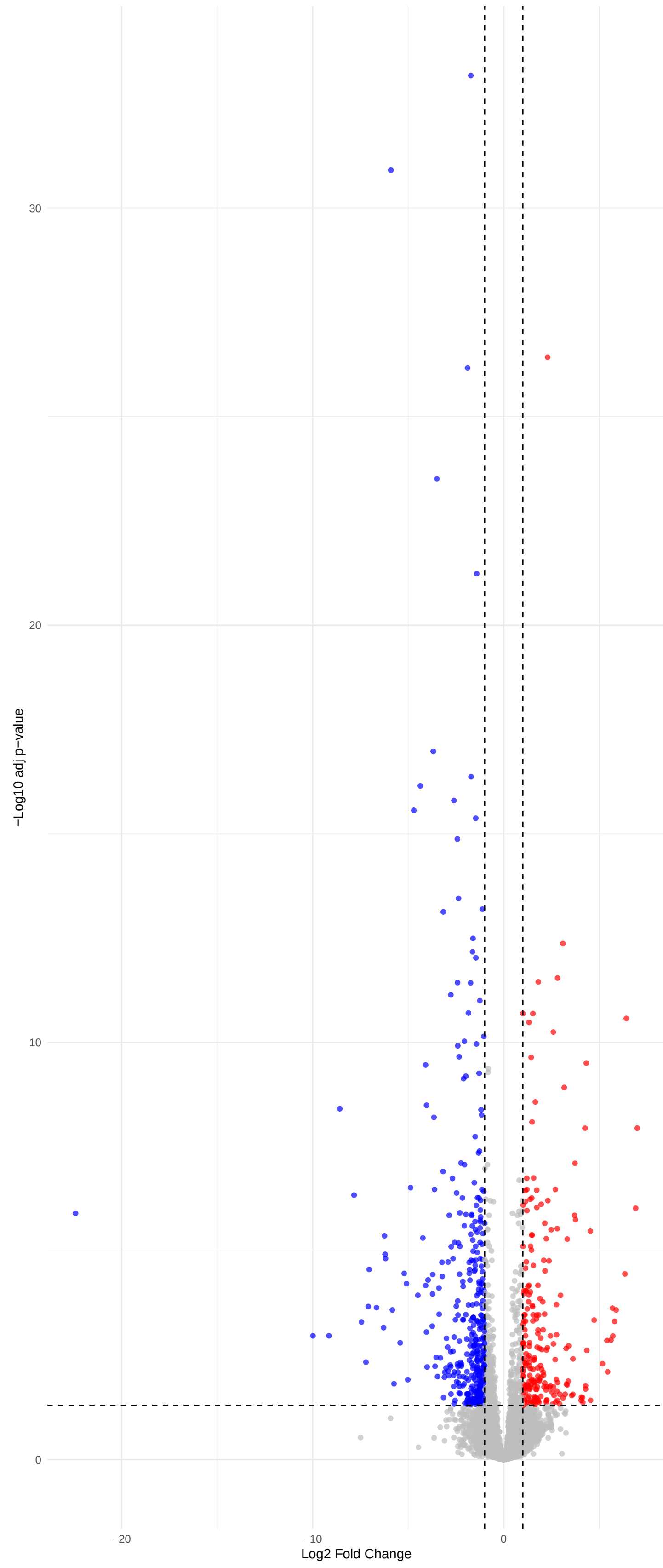
Volcano Plot: 7_WT_vs_pifq
