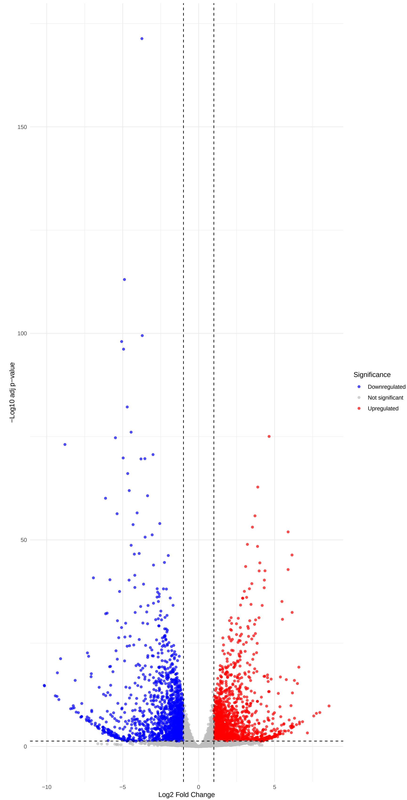
Volcano Plot: Epidermis_Cotyledon_WT_vs_pifq
