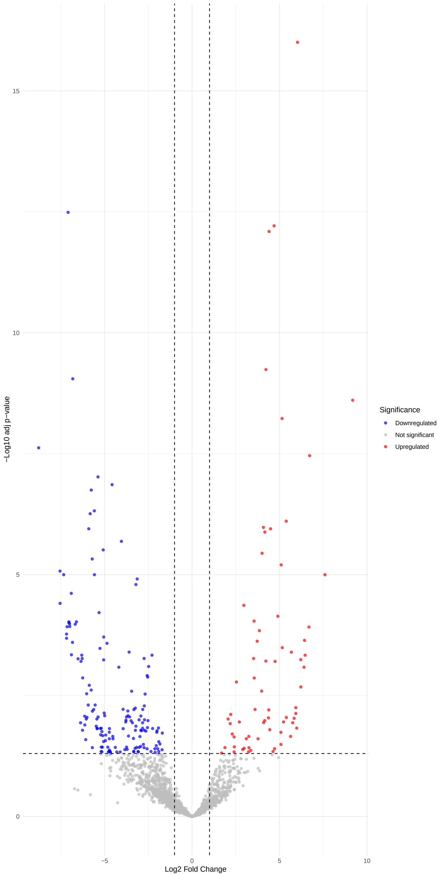
Volcano Plot: ENDO1_WT_vs_pifq
