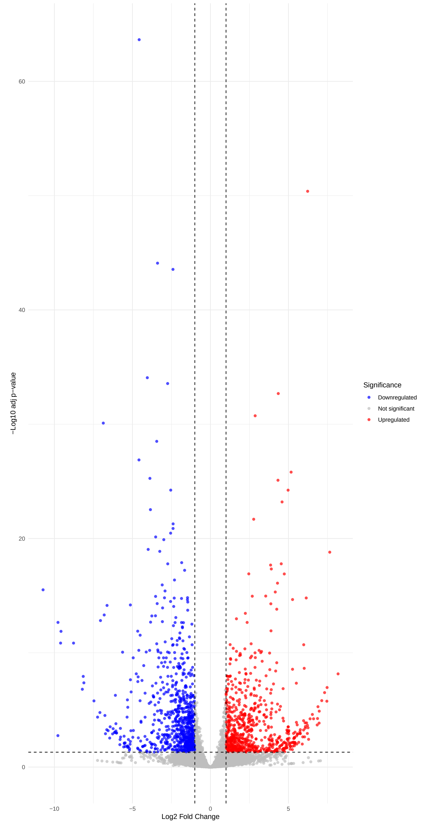
Volcano Plot: 4_WT_vs_pifq
