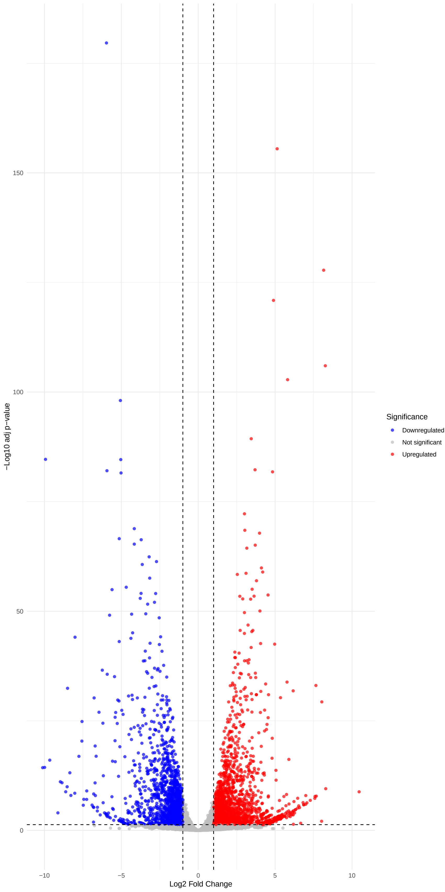
Volcano Plot: Epidermis_Hypocotyl_1_WT_vs_pifq
