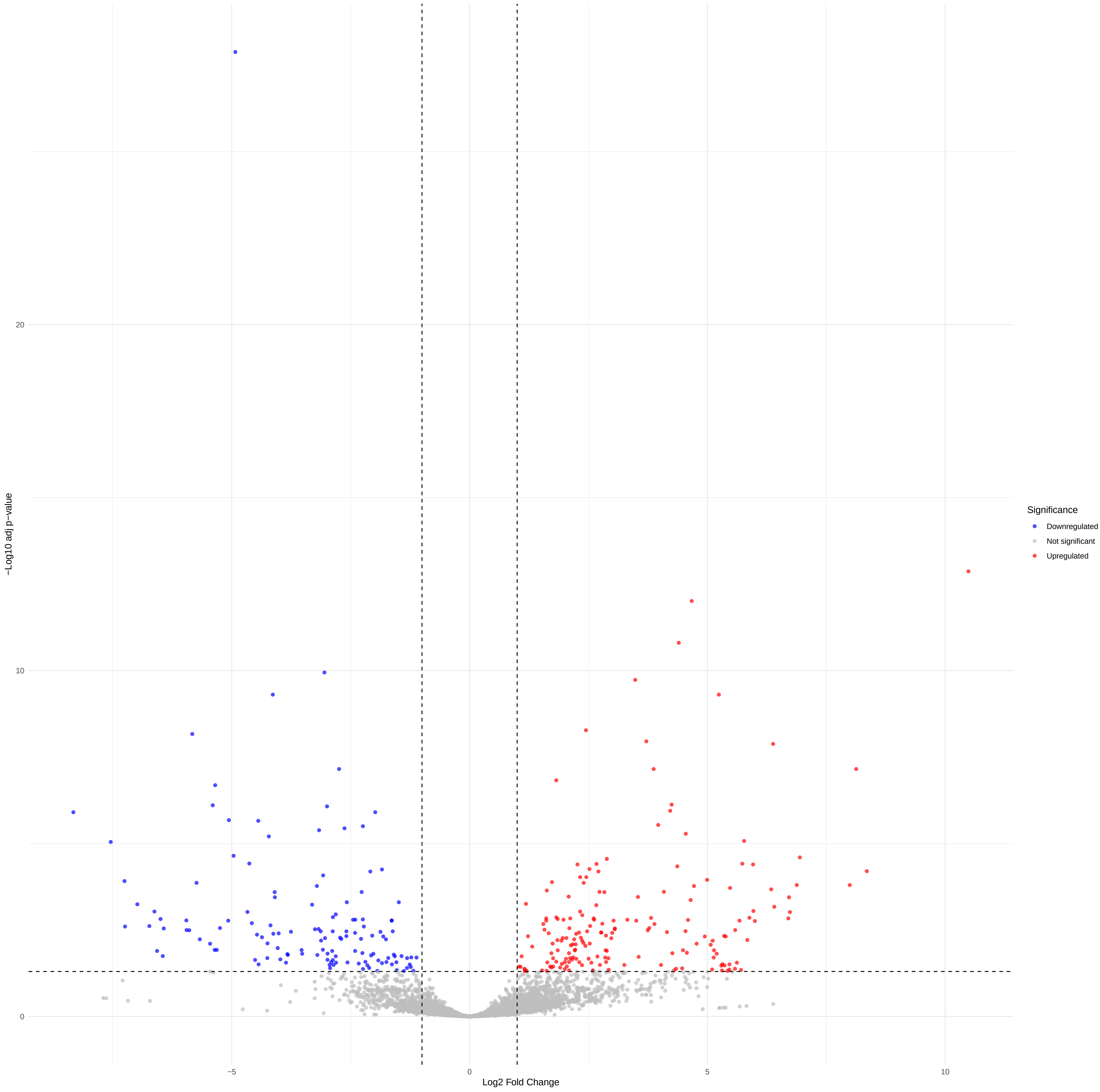
Volcano Plot: PHLOEM_WT_vs_pifq
