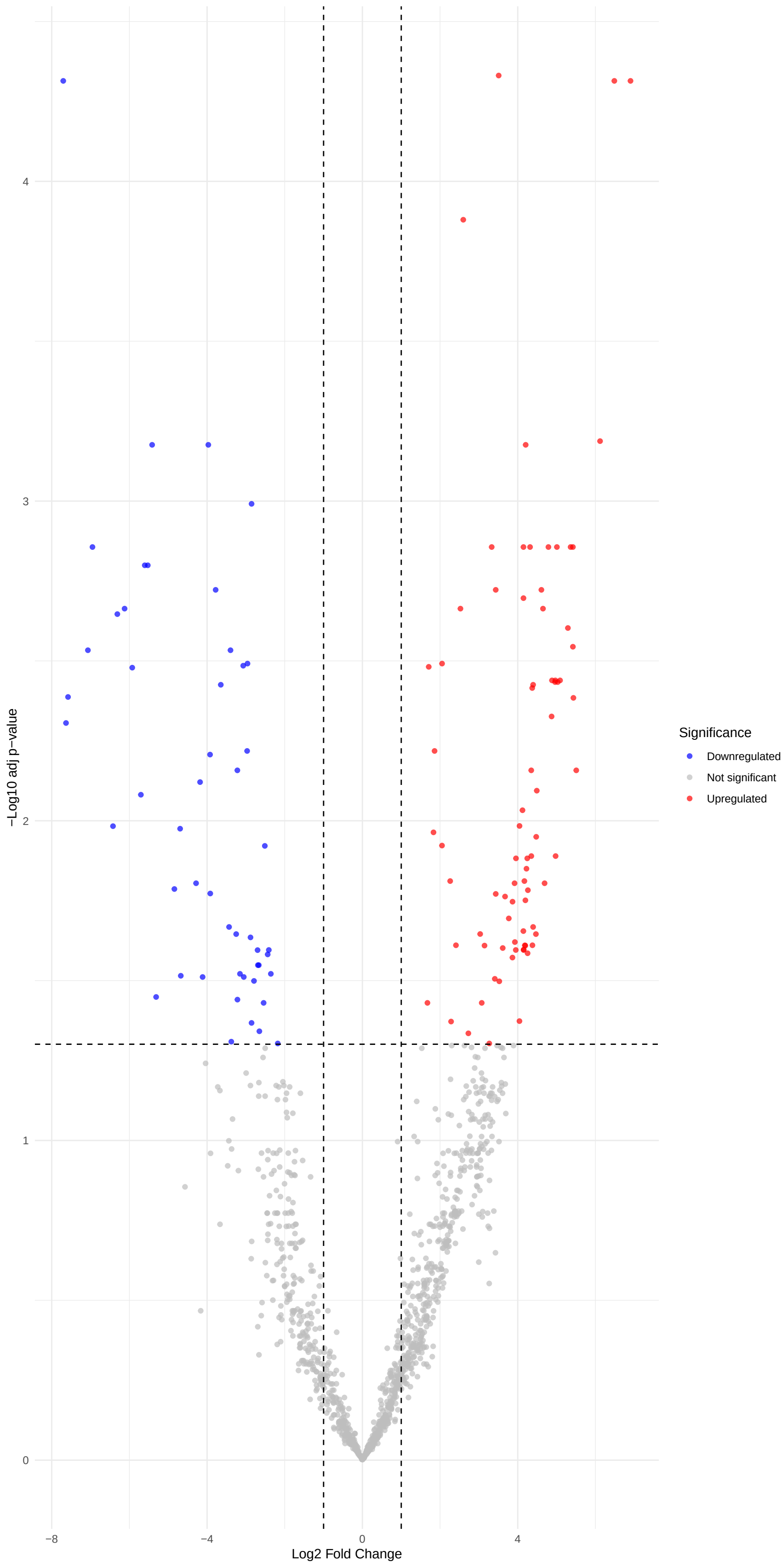
Volcano Plot: guard_cell_WT_vs_pifq
