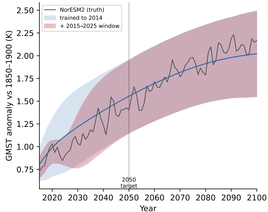
(a) FaIRGP posterior (SSP2-4.5, 95% epistemic)
