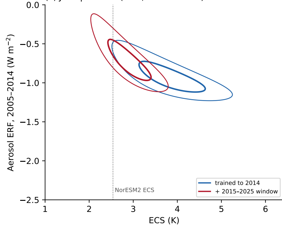
(a) Joint posterior (50%, 90% credible)
