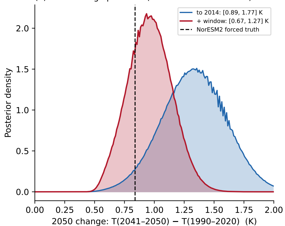
(b) 2050-change posterior (54% variance reduction)
